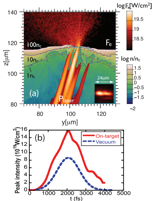
FIG. 3: (a) Snapshot of laser Poynting flux ( P_{laser} ), electron density (contour lines), and electron energy flux ( F_e ) at peak power in the 2D PIC simulation. The red dashed contour lines are at t = 0 and the blue lines are at t = 2.2 ps. The inset is a typical on-shot Titan vacuum focus. (b) Time history of incident peak intensity (blue dashed line) and actual peak intensity on target (red solid line).
