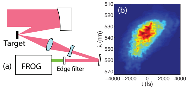
FIG. 1: (a) Setup for FROG measurements of specular light. (b) A typical specular FROG trace.
