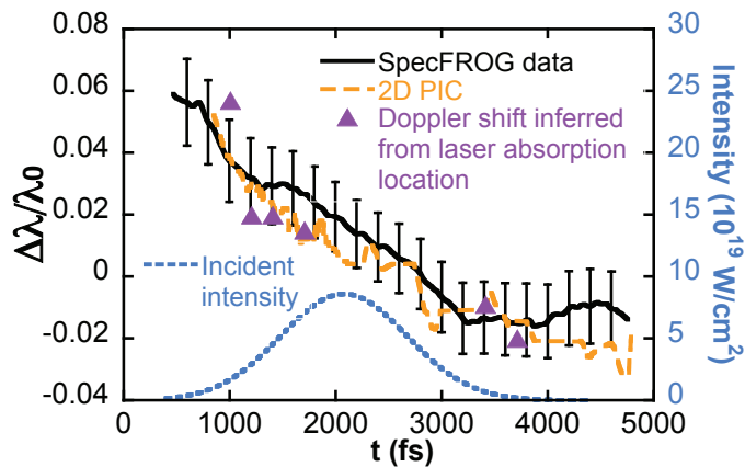
FIG. 2: Comparison of measured and simulated time history of spectral shift. Black solid line: specular FROG data. Orange dashed line: central wavelength of specular 2\omega spectrum in the 2D PIC run. Purple triangles: expected Doppler shift inferred from motion of laser absorption/reflection point in the 2D PIC run. Blue dashed line: incident vacuum peak intensity (99th percentile).
