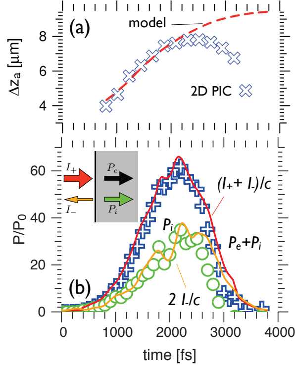
FIG. 4: (a) Motion of the laser absorption point in reduced 2D PIC simulation vs. simple model. The symbols are the locations where the laser field vanishes (uncertainties due to 2D structure are represented by the finite size). The line represents the motion predicted by Eq. (4). All positions are relative to the point where n_e(0) = n_c . (b) Momentum flux balance between laser light and plasma in units of P_0 \equiv n_c m_e c^2 \approx 1 \text{Gbar} for 1 \mu\text{m} wavelength light. The lines represent the laser momentum, and the symbols represent the electron/ion momentum.
