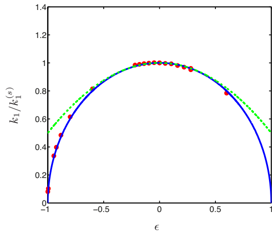
FIG. 2: (Color online) The stiffness of unpressurized ellipsoidal shells, k_1 , compared to the stiffness of a sphere with the same mean curvature \kappa_M , k_1^{(s)} , plotted as a function of the asphericity parameter \epsilon = (R_y - R_x)/(R_x + R_y) . The asymptotic expression (13) (dashed curve) agrees well with numerical results for \epsilon \ll 1 . However, the fit (14) (solid curve) gives a good account even for \epsilon = O(1) . Numerical data were obtained in simulations with t = 5 mm and b = c = 1 m.
