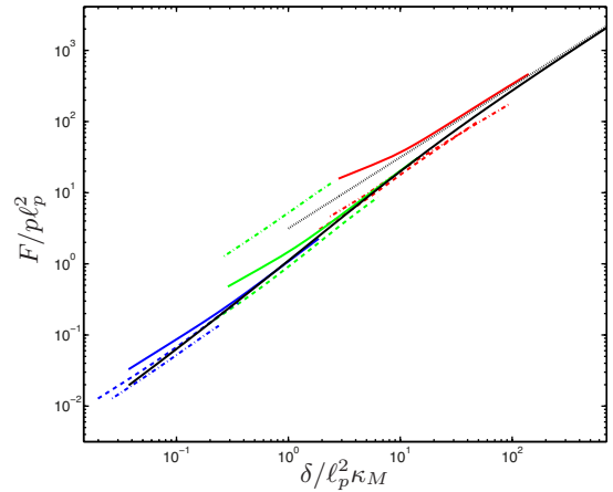
FIG. 4: (Color online) Force-displacement curves at large displacements. The results of ABAQUS simulations are shown for shells with a = 5 m, \kappa_G/\kappa_M^2 = 0.148 (dashed curves), a = 2.5 m, \kappa_G/\kappa_M^2 = 0.476 (dash-dotted curves) and a = 1 m, \kappa_G/\kappa_M^2 = 1 (solid curves). The simulated shells have thickness t = 2 mm, b = c = 1 m and a variety of internal pressures: p = 10^5 Pa (red), p = 10^6 Pa (green) and p = 10^7 Pa (blue). Here \kappa_M^{-1} is used as the radius of curvature in \ell_p . Numerical (solid black curve) and asymptotic (dotted line) results for a spherical membrane shell [5] are also shown.
