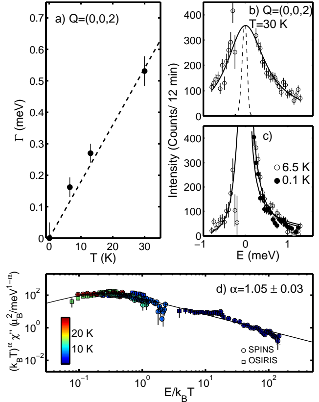
FIG. 2. (a) illustrates the linewidth of the magnetic excitations taken from constant Q scans represented in panels (b) and (c). The dashed curve in (b) centered at E=0 , is the measured resolution on SPINS. Panel (d) summarizes all of the temperature dependence from SPINS and OSIRIS and plots k_B T^\alpha \chi'' as a function of E/k_B T over the temperature range T=[0.1, 30] K (as described by the colorbar) and integrating over \mathbf{Q}=(\pm 0.1, \pm 0.1, 2\pm 0.25) on OSIRIS. The exponent \alpha was fitted to be \alpha=1.05 \pm 0.03 as described in the supplementary information.
