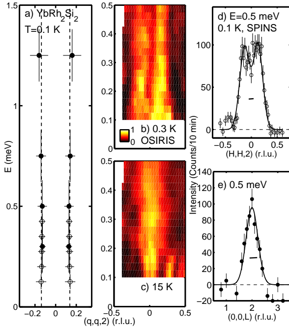
FIG. 1. The \hbar\omega - Q dependence of the magnetic fluctuations in \text{YbRh}_2\text{Si}_2 at T=0.1 K. (a) the position in Q of the ridges of scattering where filled (open) circles are from SPINS (OSIRIS). (b) and (c) plot contour maps of the spin fluctuations taken on OSIRIS at 0.3 K and 15 K integrating over the range (q,q,2\pm 0.25) . (d) and (e) show background corrected cuts in momentum at 0.5 meV. The horizontal bars are the experimental resolution.
