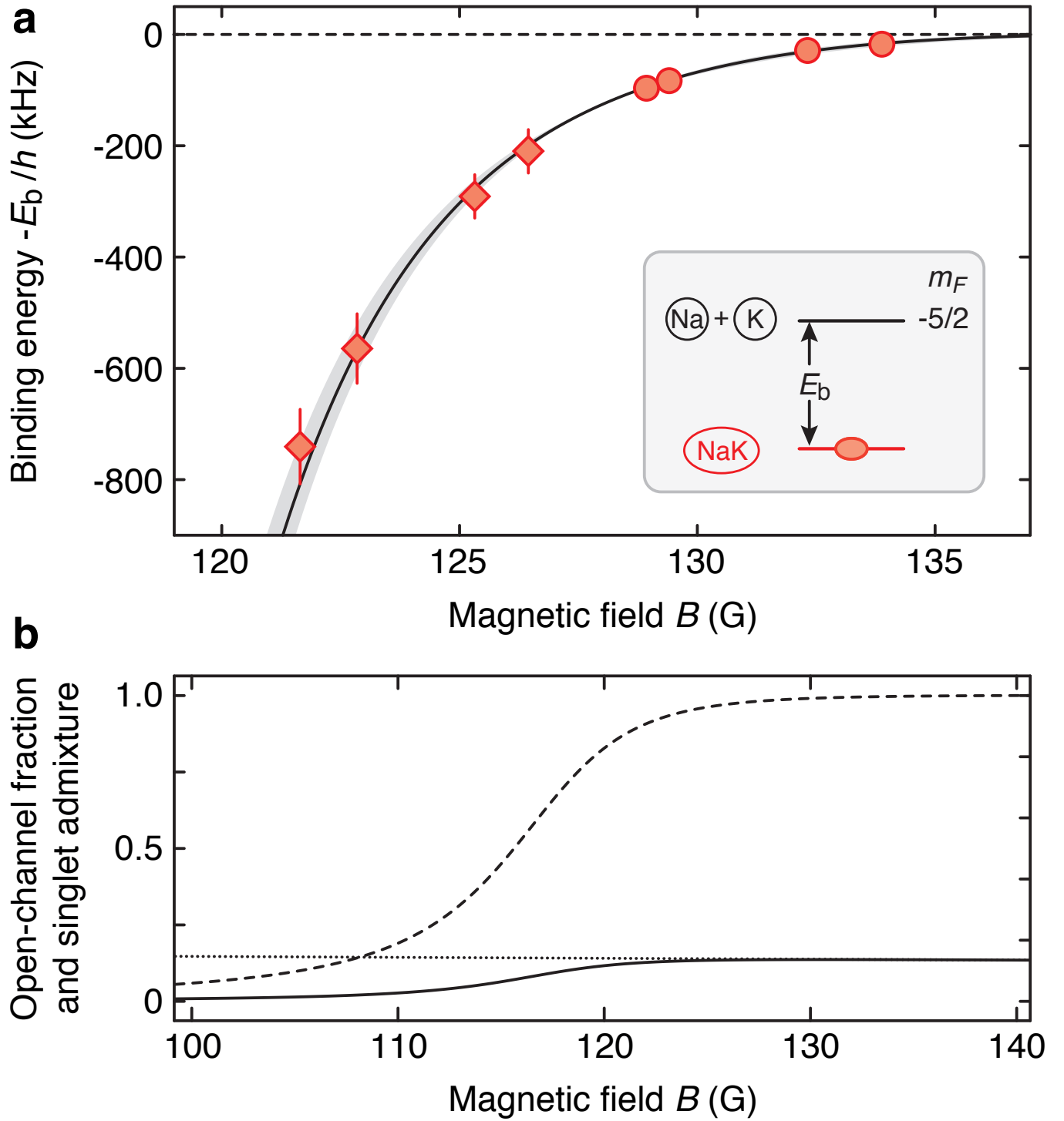
FIG. 2. (color online). (a) Binding energy of NaK Feshbach molecules at the wide Feshbach resonance between |1, 1\rangle_{\text{Na}} and |9/2, -5/2\rangle_{\text{K}} . Binding energies smaller than 200 kHz (circles) are obtained by direct detection of molecules (see Fig. 1(a)), while larger binding energies (diamonds) with weaker free-bound coupling are measured by detecting simultaneous atom loss in |1, 1\rangle_{\text{Na}} and |9/2, -3/2\rangle_{\text{K}} . The solid line is a one-parameter fit to the model described in the text, and the shaded region displays the uncertainty. (b) Open-channel fraction (dashed line) and singlet admixture of the molecular state (solid line), derived from the binding energy curve in (a), and singlet admixture of unbound pairs (dotted line).
