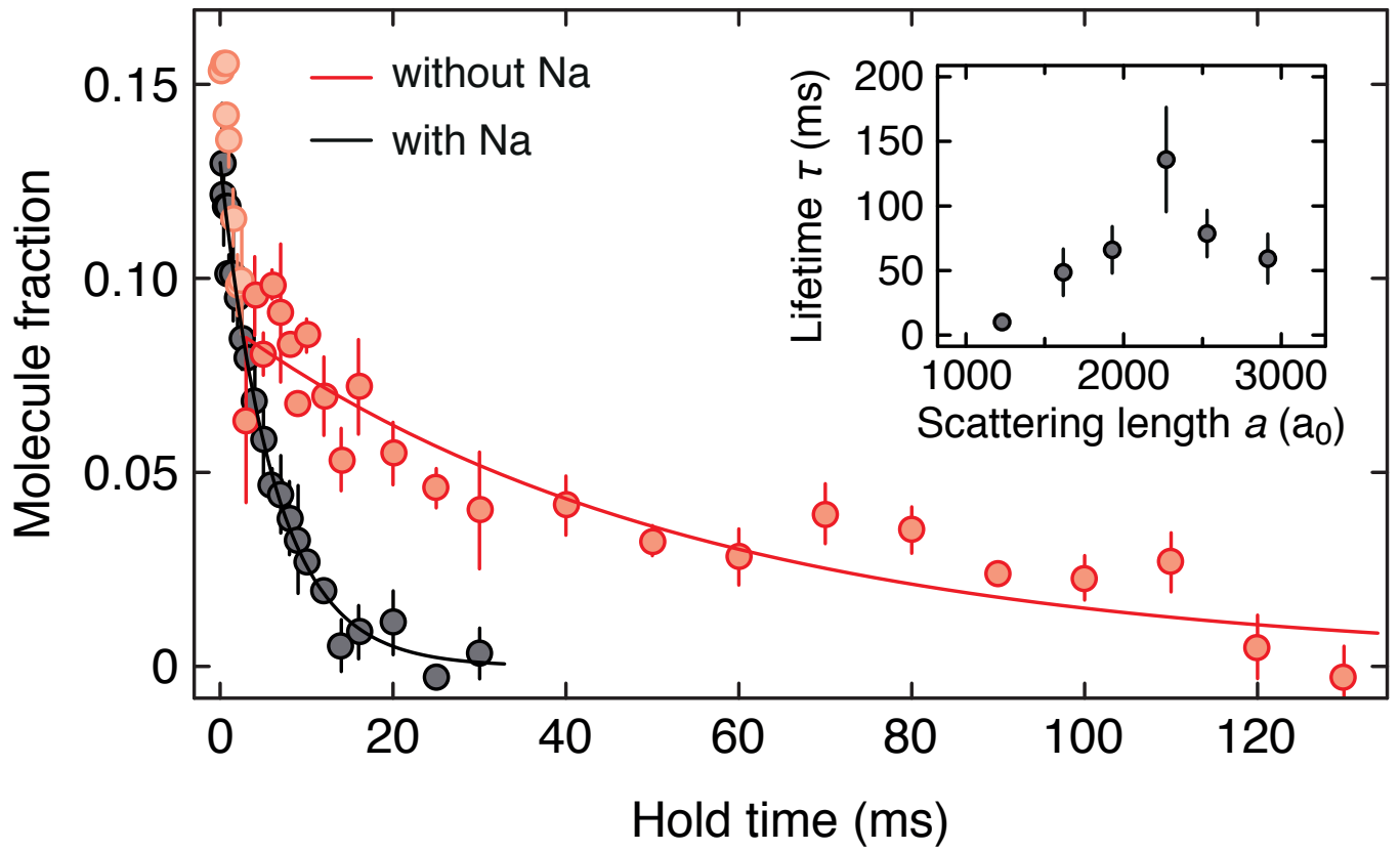
FIG. 4. (color online). Lifetime of fermionic Feshbach molecules. The measurement is performed at a magnetic field of 132.2 G, corresponding to a binding energy of 32 kHz. The red (black) data points show the number of molecules as a function of hold time with (without) removing sodium from the dipole trap directly after association. Solid lines correspond to exponential fits yielding a 1/e -time of 54(13) ms and 8(1) ms, respectively. The inset shows the lifetime as a function of the scattering length between bosons and fermions. The maximum observed lifetime is 140(40) ms.
