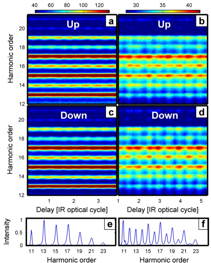
FIG. 2. Photoelectron energy spectra as a function of the time delay between the IR pulse and the APT formed by odd harmonics only (a,c), and by both odd and even harmonics (b,d). (e,f) Experimental harmonic spectrum.
