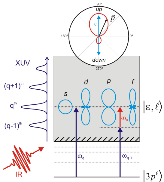
FIG. 1. Principle of the measurement.
