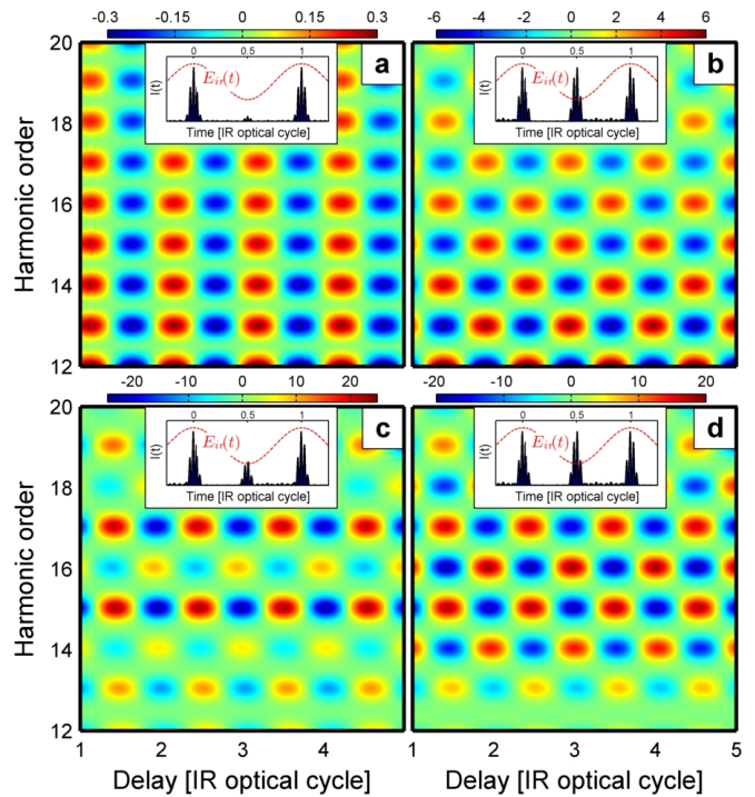
FIG. 4. Theoretical coefficient \beta_1 for different even-odd phase shifts. Top row: FSI term for (a) 0. and (b) 0.5\pi . Bottom row: Full calculation for (c) 0.35\pi and (d) 0.5\pi . Insets: temporal profile of the APTs used in the calculations.
