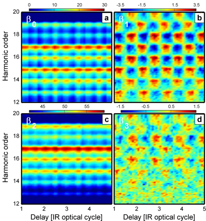
FIG. 3. Experimental expansion coefficients \beta_J associated with the first four Legendre polynomials P_J .
