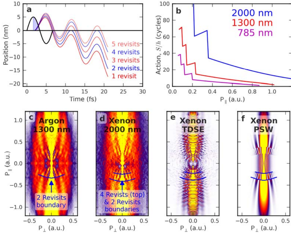
FIG 3. (a) Depending on when an electron tunnels, it will be driven past the ion a specific number of times. (b) Quantum phase obtained by integrating each electron trajectory from when it is born to when it revisits the ion for the second-to-last time versus the final momentum parallel to the laser polarization ( P_{\parallel} ). The frequency of the plane and spherical waves is given by the slope of this graph. The “steps” at low momenta correspond to regions of multiple rescattering. (c) Experimental photoelectron distribution from argon ionized by a 1.3 \mu\text{m} , 7.5 \times 10^{13} \text{ W/cm}^2 laser shows a clear boundary between the high momentum region (one revisit) and the low-momentum region where scattering can take place during a subsequent revisit. (d) Photoelectron distribution from xenon using a 2.0 \mu\text{m} , 5 \times 10^{13} \text{ W/cm}^2 laser displays two boundaries that correspond to the second and fourth revisits. (e) TDSE calculations reproduce the low-momenta structures in xenon. (f) Single-cycle PSW model, including scattering on the first revisit (outer spiders) as well as the second and fourth revisits (inner spider structures).
