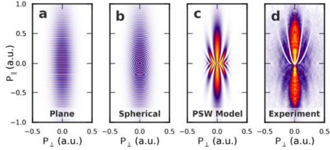
FIG 2. The plane-spherical wave model (PSW). The superposition of a plane wave (a) and a spherical wave (b) generates an interference pattern (c) that has the same shape as the spider structures. The phase of the plane wave is given by \phi_{\parallel} = k_{\parallel} z , while the phase of the spherical wave is given by \phi_{\text{sph}} = k_{\text{tot}} r - \omega t , where k_{\parallel} is the momentum parallel to the laser polarization, k_{\text{tot}} is the total momentum, and \omega is the modulation frequency of the plane and spherical waves. Only the real part of the complex wave is shown in panels (a) and (b) while \phi_{\text{tot}} is shown in panel (c). (d) The minima of the spider structure calculated using the plane spherical model (white lines) match the experimental data across a broad range of wavelengths and intensities (shown: 1300 nm, 5 \times 10^{13} \text{ W/cm}^2 , 40 fs driving laser).
