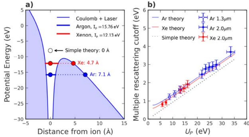
FIG 4. (a) In the presence of a strong laser field ( 5 \times 10^{13} W/cm 2 ), the atomic Coulomb potential is deformed, enabling tunnel ionization. (b) By examining the classical equations of motion, we plot the theoretical cutoff between trajectories that revisit the ion once and those that rescatter several times (lines). If the tunnel distance is included, the theoretically predicted multiple rescattering cutoffs agree with the experimentally observed cutoffs (points). The experimental intensity was calibrated from the cutoff. The error in the energy of the multiple rescattering cutoff was assumed to be 0.02 atomic units of momentum.
