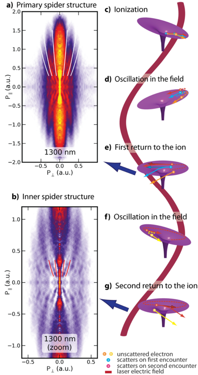
FIG 1. (a) The photoelectron angular distribution resulting from the ionization of argon gas with a 1300 nm, 7.5 \times 10^{13} W/cm 2 , 40 fs laser pulse. The primary spider structure (minima shown with white lines) results from the interference between directly ionized electrons and those that are driven back to scatter from the Coulomb potential. (b) The newly observed inner structure (minima shown with red lines) results from electron trajectories that scatter from the Coulomb potential on their second re-encounter with the ion and the interfere with unscattered trajectories. (a – e) Simple laser-driven electron dynamics during ionization explain the primary and inner spider structures.
