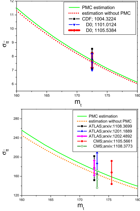
FIG. 1. Total cross-section \sigma_{t\bar{t}} for the top quark pair production versus top quark mass.
