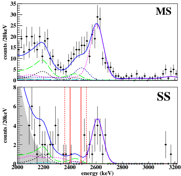
FIG. 5: Energy spectra in the ^{136}\text{Xe} Q_{\beta\beta} region for MS (top) and SS (bottom) events. The 1 (2) \sigma regions around Q_{\beta\beta} are shown by solid (dashed) vertical lines. The 0\nu\beta\beta PDF from the fit is not visible. The fit results have the same meaning as in Figure 4.
