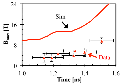
FIG. 5. B field amplitudes inferred from path-integrated measurements. The scale length of the field structure in the direction of proton propagation is approximated as the amplitude of the perturbation at each sample time.
