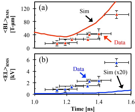
FIG. 4. Inferred path-integrated quantities ( \blacktriangle ) are calculated from measured \alpha_{RMS} values if deflections are caused by (a) B-fields and mass, or (b) E-fields and mass. Simulated B fields indicate an approximate upper estimate and are a factor of \sim 2 higher than inferred values, whereas simulated E fields are a factor of \sim 100 too low to account for measured proton fluence modulations.
