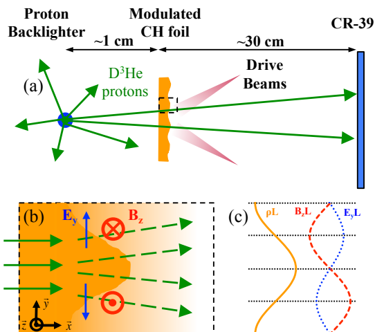
FIG. 1. (a) A schematic drawing of the experimental setup used to radiograph directly-driven plastic (CH) foils with 2D seed perturbations. Proton images are recorded on CR-39 nuclear track detectors. In x ray radiography experiments, a uranium foil backlighter was used, and images taken on film. (b) An expanded view of proton (green) deflections due to RT-induced density, E field (blue), and B field (red) modulations in the target. (c) Path-integrated quantities (arbitrary units) are shown during the linear growth phase.
