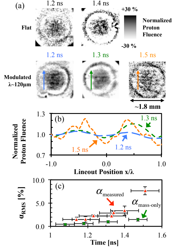
FIG. 3. (a) Sample proton fluence radiographs for flat and modulated foils; scale size is given in the target plane and lineout direction is indicated. Proton fluence is normalized for comparison across different shots. (b) Corresponding lineouts for radiographs of modulated targets. (c) Measured RMS fluence variations ( \blacktriangle ) in proton radiographs. Expected RMS variation due to mass only ( \bullet ) was calculated using density distributions from x-ray data.
