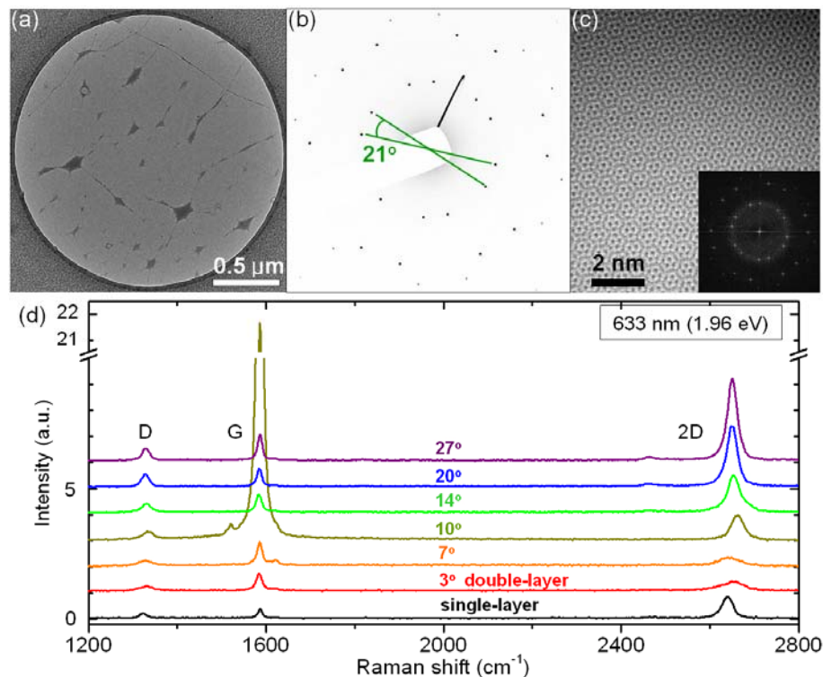
FIG. 1. (Color online) Suspended rotated double-layer graphene and Raman spectrum. (a) TEM image of misoriented double layer graphene. The graphene sample is suspended in a hole of 2 μm diameter. (b) Diffraction pattern of the graphene sample shown in (a). The two sets of hexagonal patterns are relatively rotated by 21 degrees. An electron beam size of ~ 1 μm is used for diffraction acquisition. (c) Atomic resolution TEM image of double-layer graphene with rotational angle of 21 degree showing a moiré pattern. Inset shows a fast Fourier transform (FFT) of the image. (d) Raman spectra of misoriented double-layer and single layer graphene measured with 633 nm wavelength laser (1.96 eV). The spectra are shifted vertically for clarity.
