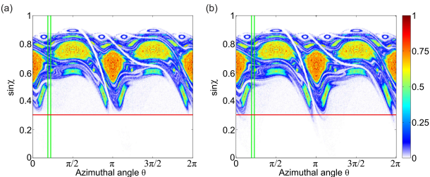
FIG. 2: Normalized survival probability for (a) transverse electric (TE) and (b) transverse magnetic (TM) polarization in cavity-waveguide system as Fig. 1(b) with n=3.3 . 40000 rays of equal intensity start uniformly above the critical angle in the SOS and their intensity evolves by the modified Fresnel Law [31]. For simplicity, we reduce the intensity of each ray to zero once it impinges on the exit window. Color represents the total intensity of rays in a tiny area around each point in the SOS. The vertical and horizontal lines indicate the exit window to the waveguide and the critical line, respectively.
