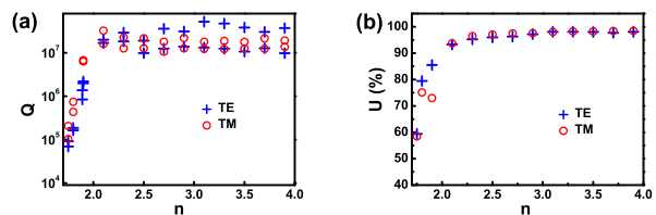
FIG. 4: Q-factor (a) and unidirectionality U (b) of mode-4 in Fig. 3(a) as a function of the refractive index.
