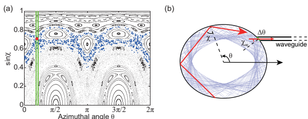
FIG. 1: (a) Poincaré SOS for a quadruple cavity at \varepsilon = 0.08 . The cavity is taken to be closed. Fine details of the SOS are removed for clarity. Light in a high-Q mode undergoes chaotic motion once it tunnels from islands into the neighboring chaotic region. The first 800 bounces of a typical trajectory outside the period-4 “diamond” islands are indicated by the blue dots, which form a chaotic “layer” around the islands. Its real space representation is shown in (b). Eventually the rays diffuse to the lower portion of the SOS, and the real space trajectory does not have a caustic in contrast to (b). Green lines in (a), (b) indicate the position of the exit window centered at \theta = 0.633 with a angular width of \Delta\theta = 0.125 . Red square in (a) marks the incident angle \chi_w of the light that enters straight into the waveguide.
