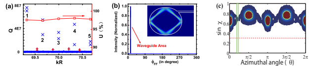
FIG. 3: (a) Resonance spectrum of the cavity-waveguide system shown in Fig. 1(b). Diamond modes are indicated by “x” and the others are marked by “+”. They appear as quasi-degenerate pairs due to the slightly different influences of the waveguide on modes of different quasi-reflection symmetry. Open squares show the unidirectionality ( U ) of modes 1-5. (b) FFP of mode-4 measured at r = 2.3R as a function of the observation angle \phi_{FF} . Inset: Corresponding mode structure ( |H_z| ). (c) Enhanced Husimi projection of mode-4. Green lines indicate the exit window into the waveguide.
