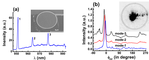
FIG. 5: (a) Measured emission spectrum from a quadruple shaped microdisk with a waveguide. Inset: top-view SEM image. (b) Measured FFPs of the three lasing modes shown in (a). Top two lines of mode-2 and mode-3 are shifted vertically 0.2 and 0.4 for clarity, and each line is normalized by its peak intensity. Inset: Top-view microscope image of mode-1. Dark regions indicate strong intensity and the dashed ring shows the position of the measurement ring, the scattering from which is measured to give the emission pattern.
