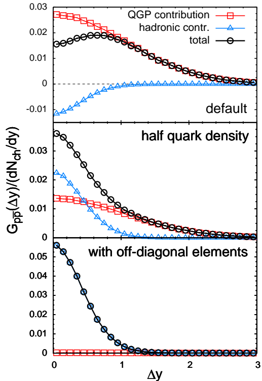
FIG. 2. Correlations involving other hadronic species are more effective at separating the QGP and hadronization components because the two components might contribute with opposite signs. Such is the case for the p\bar{p} and pK^- correlations shown in the upper panels of Figs. 2 and 3, respectively. The dip in the p\bar{p} correlation and the switch of signs in the pK^- correlation only exist if there are competing correlations of opposite sign. Proton-antiproton correlations test the idea that charge production comes in two separate waves, because the hadronization and QGP contributions have opposite signs as seen in the upper panel. The middle panel illustrates the sensitivity to reducing the diagonal elements of \chi_{ab}^{(\text{QGP})} by a factor of two, and the effect of adding large off-diagonal components as in Eq. (10) is displayed in the lower panel.
