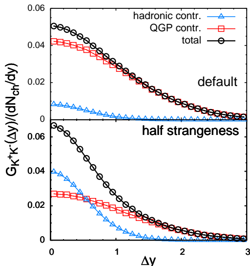
FIG. 4. Since few strange quarks are produced during hadronization, the hadronization component for K^+K^- correlations is small as shown in the upper panel. If the QGP had half the strangeness content, the hadronization component would be larger and one would have a much narrower correlation as seen in the lower panel.
