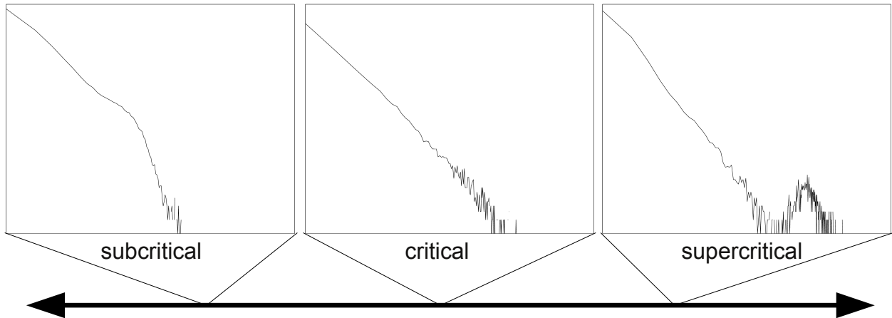
Figure 4: Avalanche size histograms from three different samples of rat cortex. The horizontal line represents a path in some representative (such as increasing mean connection strength or increasing number of connections) direction in the complex parameter space of network, representing how critical the sample of interest is. As we move along this path towards greater network connectivity, samples change from having early exponential cut-offs, to straightforward power laws, to having humps in their distribution. These humps could be caused by the possibility that the finite system size, rather than the degree of network connection, is constraining the size of the largest events. These histograms show that different samples exist at different points in the phase diagram. such as the mean connection strength with fixed network topology. toward increasing excitability. Factors that determine the phase of a given sample include number of connections and connection strength. Simulations using a mean field (all-to-all connectivity) version of our model can move along the phase diagram by increasing connection strength [18, 19]. Experiments have used drugs to move the network along this line in the parameter space. [2, 20, 21].
