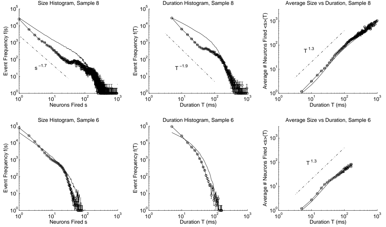
Figure 2: Contrasting size and duration distributions, and average size for fixed duration from a critical data set (top) and a subcritical data set (bottom). Experimental data is shown by lines with markers and data from the corresponding models is shown by smooth lines. Note that each experimental data set has its own simulation as we use information from the experiment to determine the parameters of the simulation (see SI). The dashed lines in the top (near critical) row correspond to power laws with exponent 1.7, 1.9 and 1.3, corresponding to the critical exponents \tau , \alpha , and 1/\sigma\nu z respectively. These values satisfy the exponent relation \frac{\alpha-1}{\tau-1} = \frac{1}{\sigma\nu z} , as is expected for a system near criticality. Statistical error bars are only significant for the largest and longest events for the experimental data, and are too small to see in the figure for the simulations
