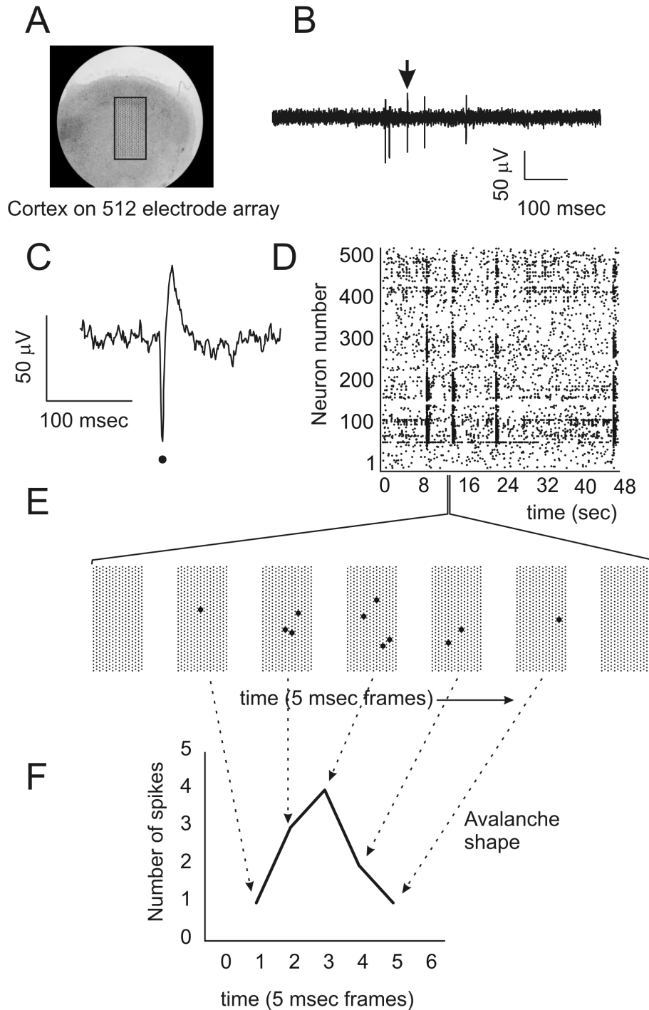
Figure 1: Recording avalanches from cortical tissue. A , Micrograph of cultured cortical slice on 512 electrode array. Black rectangle (1 mm x 2 mm) added to highlight location of array. B , Voltage trace from one electrode. Arrow marks a spike from an individual neuron, expanded in C . Time of spike is marked by black dot. D , Raster plot of spike times (dots) from many neurons over a 48 s interval. Recordings lasted up to 8 hrs. E , Expanded view of network activity reveals an avalanche. Each frame represents the array at one 5 ms bin. Small dots are electrode locations; large dots are spikes on array. An avalanche consists of consecutively active frames, bracketed by inactive frames, as shown here. F , Avalanche shape is obtained by plotting the number of spikes in each frame versus time.
