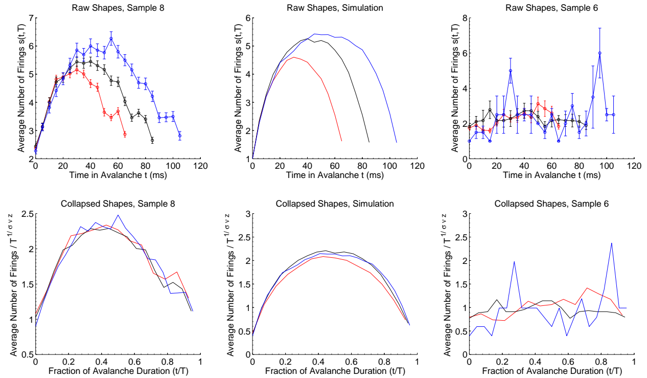
Figure 3: Avalanche shape collapses. Shapes and attempted collapses from three data sets, two experimental and one simulated. Shapes are produced by averaging the temporal profiles of all avalanches of a particular duration; different colors here represent different durations. The collapses are plotted by rescaling the horizontal and vertical axes. The left and right most data correspond to experimental data close to and far from criticality respectively (note these are the same data sets used in Figure 2). Sample 8 clearly shows the roughly parabolic shapes in the raw data, and a corresponding very clean collapse, as would be expected from critical data. Sample 6 shows neither. The middle plots are a simulation of sample 8, using TE data from that set. They clearly show similar shapes and collapse to a universal scaling function.
