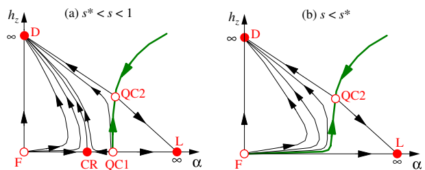
FIG. 4: Schematic RG flow for SBM2 in the \alpha - h_z plane ( h_x = h_y = 0 ). The thick lines correspond to continuous QPT; the full (open) circles are stable (unstable) fixed points, for labels see text. a) s^* < s < 1 : CR is reached for small \alpha and h_z = 0 , it is separated from L by a QPT controlled by the multicritical QC1 fixed point. Eq. (6) implies that CR is located at \alpha^* = 1 - s + \mathcal{O}[(1 - s)^2] . For finite h_z , a QPT between D and L occurs, controlled by QC2. b) 0 < s < s^* : both CR and QC1 have disappeared, such that the only transition is between D and L.
