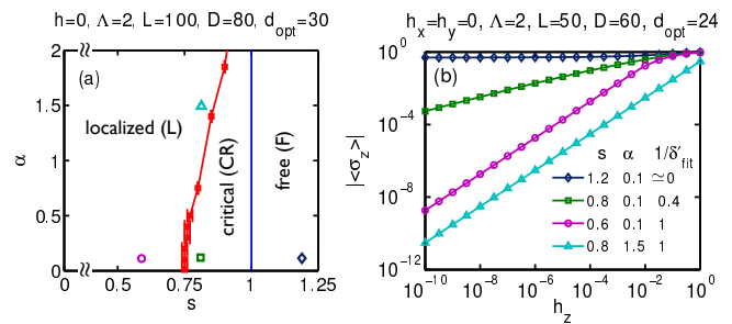
FIG. 3: a) Phase diagram of SBM2 in the s - \alpha plane for \vec{h} = 0 , with dissipation strength \alpha \equiv \alpha_x = \alpha_y . The critical phase only exists for s^* < s < 1 , and its boundary \alpha_c \rightarrow \infty for s \rightarrow 1^- . (Ref. 18 describes the determination of the phase boundary and gives a 3D sketch of the s - \alpha - h_z phase diagram, see Fig. S8.) b) Transverse-field response of SBM2, \langle \sigma_z \rangle \propto h_z^{1/\delta'} , for four choices of s and \alpha , showing free (diamonds), critical (squares) and localized (triangles, circles) behavior.
