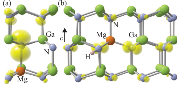
FIG. 1: (Color online) (a) Local structure showing the distortion around a neutral Mg acceptor in GaN. The localization of the hole on the axial nitrogen neighbor is illustrated by the spin-density isosurface (yellow), set to 5% of the maximum. (b) Structure of the Mg-H complex in GaN in the positive charge state. The spin density shows the more delocalized nature of the complex. Large green spheres denote Ga atoms, medium light blue spheres N atoms, and the orange (darker) sphere denotes the \text{Mg}_{\text{Ga}} .
