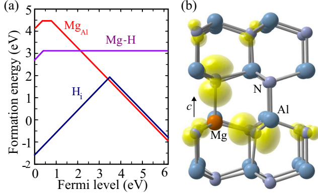
FIG. 3: (Color online) (a) Formation energy versus Fermi level for the Mg acceptor, H interstitial, and their complex in AlN. (b) Structure and spin-density associated with the localized hole states ( S=1 ) of Mg_{Al}^+ (isosurface at 5% of the maximum in yellow). Large blue spheres denote Al atoms, medium light blue spheres N atoms, and the orange (darker) sphere Mg_{Al} .
