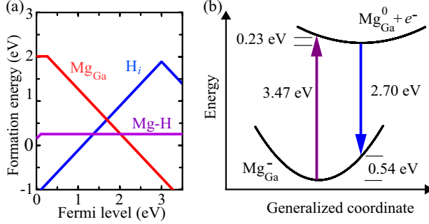
FIG. 2: (Color online) (a) Formation energy versus Fermi level for the Mg acceptor ( Mg_{Ga} ), hydrogen interstitial ( H_i ), and their complex ( Mg-H ) in GaN. (b) Configuration coordinate diagram illustrating optical processes related to Mg in GaN. Recombination of an electron at the CBM with Mg_{Ga}^0 leads to emission peaking at 2.70 eV, explaining BL in GaN.
