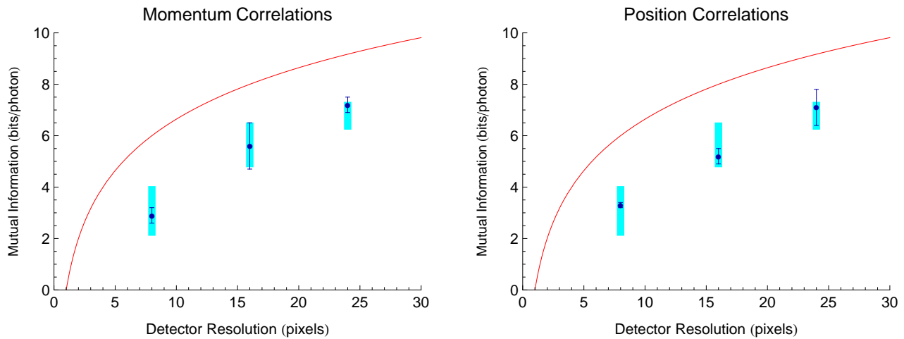
FIG. 2: (color online) Mutual Information Data. Mutual information for position correlation measurements and momentum correlation measurements are shown as a function of detector resolution. Data for detector resolutions of 8 \times 8 pixels, 16 \times 16 pixels, and 24 \times 24 pixels are shown. The dark blue points with error bars are experimental data. The light blue bars are numerical simulations based on equation 10 both for the case of perfectly relative transversely aligned detectors and the case of a relative transverse misalignment of half a pixel. The red curve is the maximum mutual information that can be detected for the number pixels per detector.
