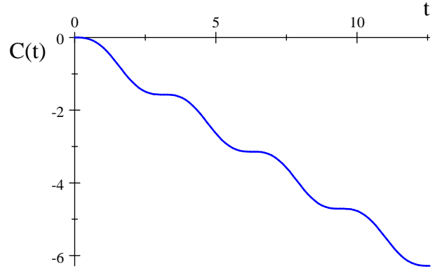
FIG. 2: Monotonic flow for the SHO C(t) .
