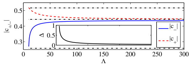
FIG. 2: (Color online) Using r = 1.2 , |c_-| (solid blue) and |c_+| (dashed red) versus \Lambda from an initial profile with \Lambda = 10 . Inset: \Delta .
