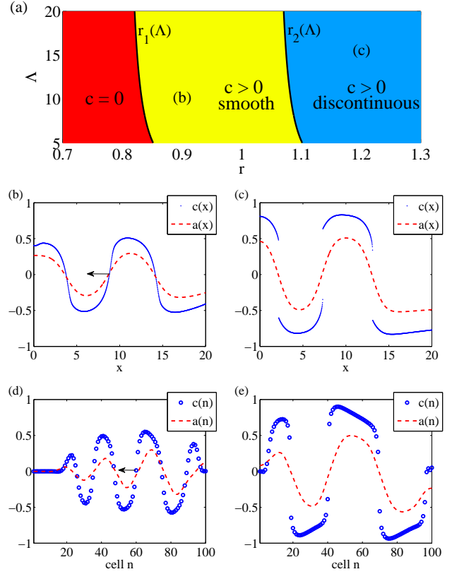
FIG. 1: (Color online) (a) Nature of steady-state solutions in the r - \Lambda plane. From left to right, no alternans ( c = 0 ), smooth calcium profiles ( c > 0 , smooth), and discontinuous calcium profiles ( c > 0 , discontinuous). (b) Smooth traveling and (c) discontinuous stationary c(x) (blue) and a(x) (dashed red) profiles from simulating Eqs. (7)-(9), using (r, \Lambda) = (0.9, 10) and (1.2, 15) , respectively. Alternans profiles obtained from a detailed ionic model [15] analogously showing (d) smooth traveling and (e) discontinuous stationary solutions.
