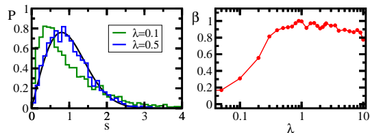
FIG. 1: Left: P(s) for Model 2 with \lambda = 0.1, 0.5 compared with the Wigner-Dyson distribution (smooth curve). Right: Brody parameter \beta as a function of \lambda .
