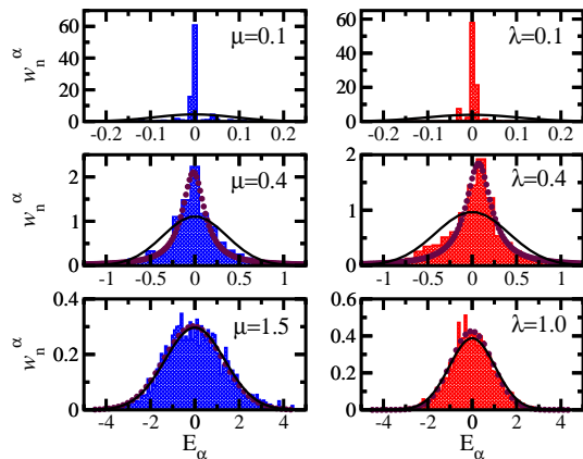
FIG. 3: (Color online) Strength functions for Model 1 (left) and Model 2 (right) obtained by averaging over 5 close states in the middle of the spectrum. Middle panels : circles give a Breit-Wigner fit. Lower panels : circles stand for a Gaussian fit. In all panels, solid curves correspond to the Gaussian form of the energy shells.
