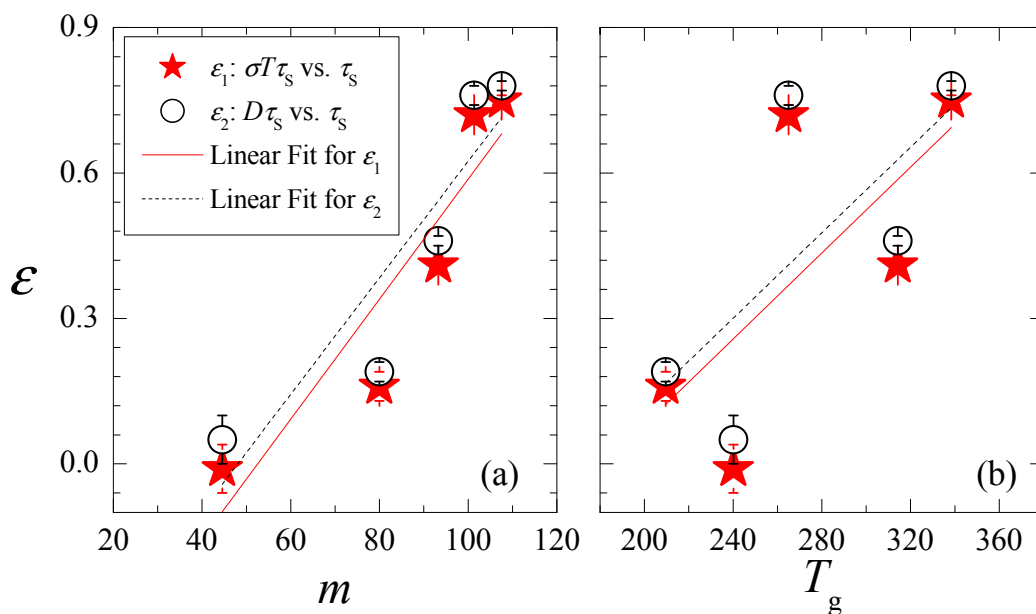
FIG. 4 (color online). Correlation between the decoupling exponent \varepsilon and (a) the fragility index m , and (b) the glass transition temperature T_g . The fragility index is estimated from the VFT fittings parameters: m = (\ln 100 - \ln \tau_0)[T_\tau(\ln 100 - \ln \tau_0) + B_\tau]/(2.303B_\tau) . Solid lines: linear fits for \varepsilon_1 ( \sigma T \tau_S vs. \tau_S ) vs m (a), and vs T_g (b). The coefficient of determinations R^2 for m and T_g are 0.80 and 0.31, respectively. Dashed lines: linear fits for \varepsilon_2 ( D \tau_S vs. \tau_S ) vs m (a), and vs T_g (b). The corresponding R^2 for m and T_g are 0.78 and 0.33, respectively.
