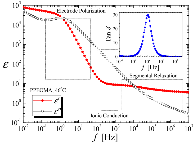
FIG. 1 (color online). Dielectric spectrum for PPEOMA at 46°C. The relaxation in the high-frequency region corresponds to the segmental motion of PPEOMA, whereas the low-frequency process is due to the electrode polarization effect. Inset: corresponding loss \tan \delta .
