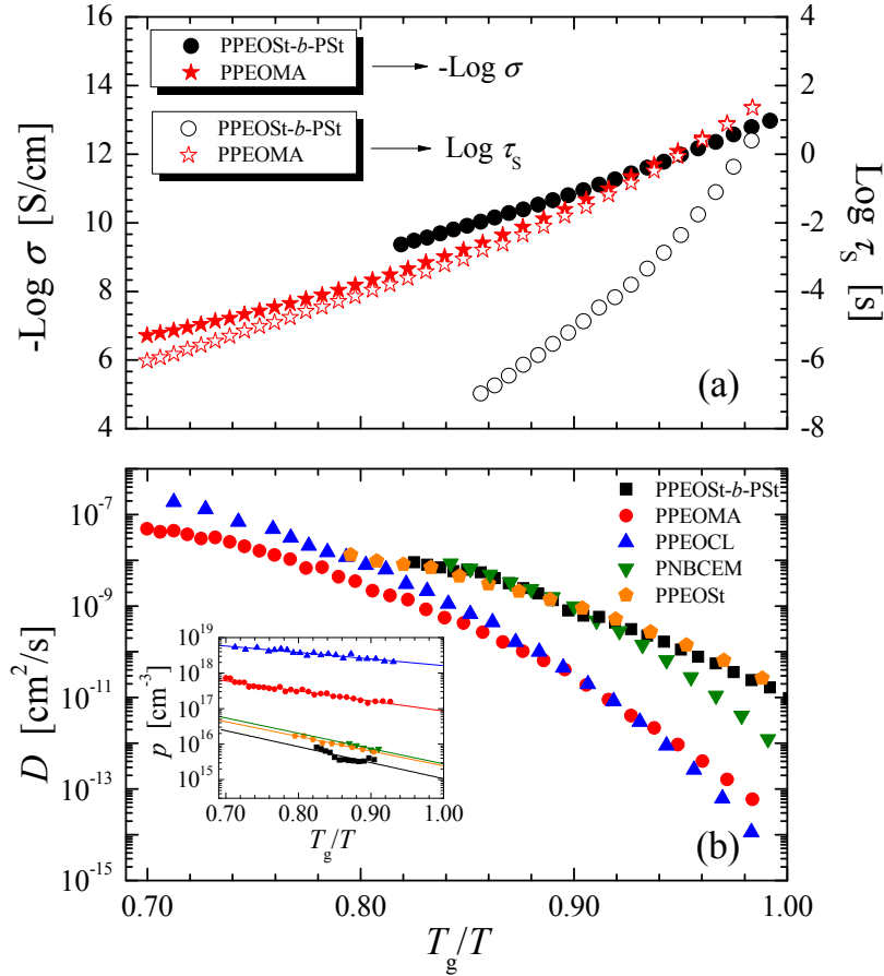
FIG. 2 (color online). (a) Temperature dependence of -\log \sigma and \log \tau_s for PPEOSt- b -PSt and PPEOMA. Solid symbols: -\log \sigma . Open symbols: \log \tau_s . (b) Temperature dependence of the ionic diffusion coefficient D obtained from \sigma and Arrhenius behavior of free ion concentration p . Inset: temperature variation of the free ions concentration (symbols), and its approximation by the Arrhenius fit (solid lines). The free ion concentration p has been corrected by certain constants such that p approaches its stoichiometric value in the high temperature limit, and D has also been adjusted accordingly. The T_g for the polymer electrolytes: PPEOSt- b -PSt, 338K; PPEOMA, 240K; PPEOCL, 210K; PNBCEM, 314K; PPEOSt, 265K. They are evaluated from the VFT equation as the temperature at which \tau_s = 100 s.
