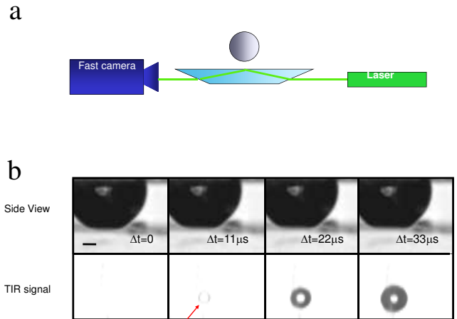
Figure 1: : Experimental setup. (a) Schematic of TIR microscopy. (b) Four typical images of a 2.6-mm-diameter drop, falling from H = 21 cm viewed simultaneously from the side and with TIR. Scale bar is 400 \mu\text{m}
