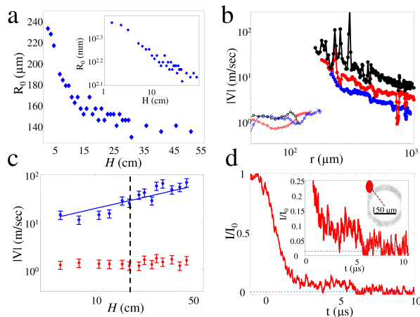
Figure 4: The initial dynamics of the wetting. (a) R_0 , as a function of H (inset) same as main figure in log scale. (b) The inwards (solid circles) and outwards (open circles) velocity of the spreading liquid for H = 26, 126, 456 mm corresponding to blue, red and black respectively. (c) Peak velocities for the outwards (blue circles) and inwards (red circles) fronts. Blue curve is the theoretically predicted initial outwards spreading velocity [18]. The dashed line indicates the threshold height above which splashing is observed. (d) A photodiode trace acquired at 100MHz measuring the intensity of the reflected light directly underneath the thin air film at a location marked by a red spot in the inset, for H = 21 cm. The dashed blue line marks the measurement noise floor. (inset) Close up of the low intensity region. The image shown is a direct visualization of the thin film of air separating the liquid from the surface prior to contact.
