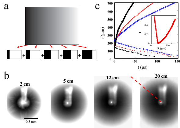
Figure 3: Virtual Frame Technique (VFT). (a) 1D schematic demonstrating the concept. Individual binary images, below, are integrated to yield the total gray-scale image. The gray scale can be interpreted to yield the time evolution. (b) Four VFT images taken at different values of H . Each image exhibits a square-shaped whiter region through the top center resulting from spurious reflections in the beam path; they are ignored in our analysis. (c) The intensity is converted to time and azimuthally averaged around the impact center. The distance of the wetting fronts from the center are plotted as a function of time for three typical experiments with H = 26, 126, 456 mm for blue circles, red pluses and black triangles respectively.
