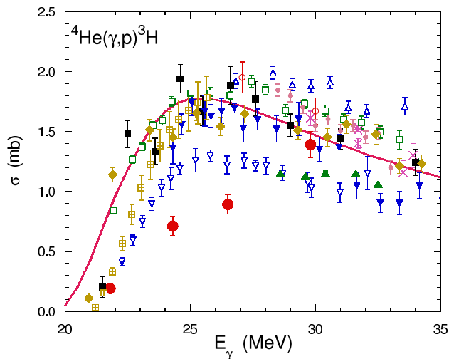
FIG. 1: (Color online) Existing data for the photodisintegration cross section of the reaction {}^4\text{He}(\gamma, p){}^3\text{H} in comparison to the calculation of the Trento group [9]. The data shown by solid symbols were obtained with bremsstrahlung beams, except for the data of Shima et al. [11] (large solid dots) and Bernabei et al. [12] (upside solid triangles), which were obtained with mono-energetic photon beams. The data indicated by open symbols are from the radiative capture reaction {}^3\text{H}(p, \gamma){}^4\text{He} using the principle of detailed balance. The data given by crosses [13] were obtained with an incident electron beam. Symbols and references for the other data are: solid squares [14], solid diamonds [15], downside solid triangles [16], small solid dots [17], open squares with inside cross [18], open squares [19], upside open triangles [20], open dots [21], downside open triangles [22].
