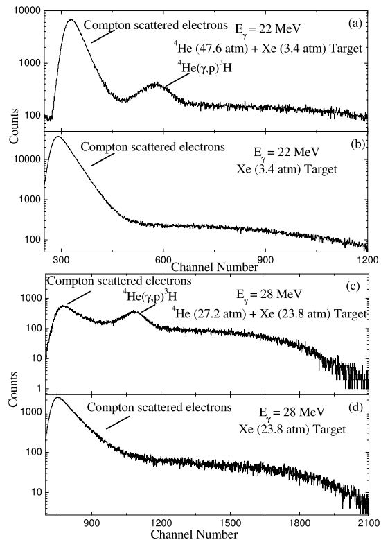
FIG. 2: Spectra for incident \gamma -energies E_\gamma = 22.0 MeV ((a) and (b)) and 28.0 MeV ((c) and (d)). Notice the logarithmic vertical scales.
