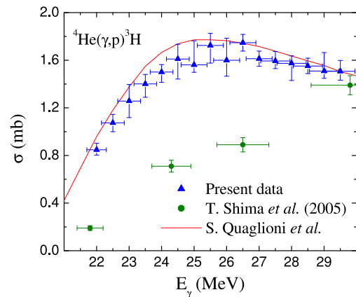
FIG. 3: Color online) Present results (triangles with error bars) for the total cross section of the reaction {}^4\text{He}(\gamma, p){}^3\text{H} in comparison to the data of Shima et al. [11] (dots with error bars), and the theoretical calculation of the Trento group [9]. The horizontal error bars are a measure of the energy spread of the incident mono-energetic photon beams. Our data at energies above 27.0 MeV were corrected for events originating from the three-body and four-body photodisintegration reactions {}^4\text{He}(\gamma, pn){}^2\text{H} and {}^4\text{He}(\gamma, 2p2n) , respectively, which are estimated to contribute to the measured yield between 27.5 MeV and 29.5 MeV at the 0.5% to 2.5% level, respectively.
