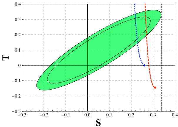
FIG. 1: Precision electroweak fit. The inner (outer) ellipse is the 95% (99%) confidence level allowed region in the S , T plane with reference Higgs mass 120 GeV [19]. The dotted blue (dashed red) line corresponds to models with a light Higgs at 130 (350) GeV, with f = 100 GeV, \tan \beta = 2 , and B\mu = 0 . The lines end when \lambda_u v_u \simeq \lambda_d v_d , where T is dominated by the light Higgs contribution. The dot-dashed black line is for the model with no light Higgs. The plot assumes that the UV contribution to the S parameter is given by the QCD value, while the UV contribution to the T parameter is estimated using NDA.
