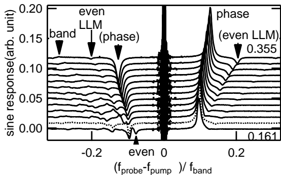
FIG. 5. Sine component of the experimental probe response near by the lower bifurcation frequency. Spectra are ordered by the pump frequency from 0.355 to 0.161 in 0.016 step. The large peak at the center is the pump signal. The lower bifurcation takes place at 0.148. The large positive amplitude identifies the soft phase mode oscillation of the ILM, the corresponding negative peak is its four wave mixing partner. The even LLM, activated by asymmetric heating of the ILM, appears as an amplitude modulation response. As the driver frequency is decreased the highest frequency band mode of the array, identified with an arrow, approaches the partner of the soft phase mode. (Lower frequency band modes appear as a sequence of positive and negative peaks.) Near the transition the even LLM frequency crosses the soft phase mode partner, dashed curve, second from the bottom. The transition takes place when the soft mode partner intersects the lower frequency odd symmetry band mode.
