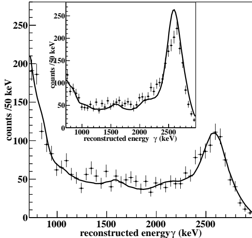
FIG. 2: Energy spectrum for a ^{228}\text{Th} calibration source at the mid-plane of the TPC, 3 cm outside the LXe volume. The intensity (vertical scale) is not fit: the agreement between the Monte Carlo (solid line) and the data tests the accuracy of the simulation against the absolute, NIST traceable, source activity. The energy scale (horizontal axis) has been corrected for \tau_e at the time of collection and has had separate energy calibrations applied for single- (main plot) and multiple-cluster (inset) interactions.
