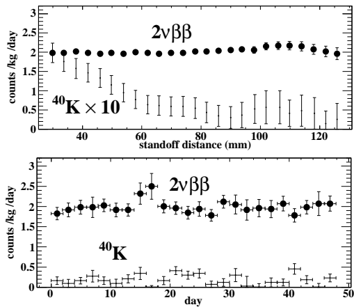
FIG. 5: Top: measured 2\nu\beta\beta decay rate of ^{136}\text{Xe} (large points) and largest background contribution ( ^{40}\text{K} , small points) as a function of the standoff distance from detector components. Bottom: event rates of 2\nu\beta\beta and ^{40}\text{K} decays as a function of time.
