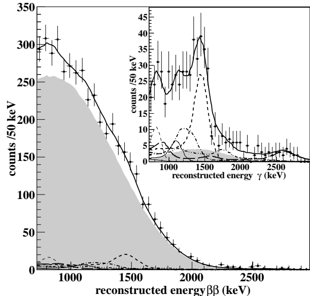
FIG. 4: Energy distributions from 752.66 hrs of EXO-200 single site events (main panel) and multi-cluster events (inset). The result of a likelihood fit to a model including the 2\nu\beta\beta decay and several backgrounds is shown (solid line) along with the 2\nu\beta\beta component (shaded region) and some prominent background components at the radius of the TPC vessel ( ^{232}\text{Th} , long dash; ^{40}\text{K} , dash; ^{60}\text{Co} , dash-dot; ^{54}\text{Mn} , thin dash; ^{65}\text{Zn} , thin solid; ^{238}\text{U} chain in equilibrium, dash double-dot). Other background components fitting to negligible amounts are not shown, for clarity. The energy scale used for the main panel is consistent with that of single-cluster, \beta -like events while the scale of the inset is consistent with the multi-cluster events it represents. The combined \chi^2/\text{n.d.f.} between the model and the data for the two binned distributions shown here is 85/90.
