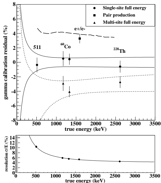
FIG. 3: Top: fractional residuals between the energy calibration points and the linear model discussed in the text. The single- (solid line) and multi-cluster (dotted line) uncertainty bands are systematic, stemming from the finite accuracy of the position reconstruction and the \tau_e correction. The thick dashed line represents the central value of the shift predicted by the simulation for point-like energy depositions. Bottom: measured energy resolution (points) along with a parameterization (line).
