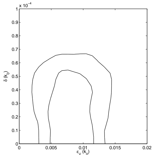
FIG. 2. 2D marginalized distribution for the quantum-gravity parameter \delta(k_0) = \alpha_0\delta_{\text{PI}}(k_0) and the slow-roll parameter \epsilon_V(k_0) with the pivot k_0 = 0.002 \text{ Mpc}^{-1} for n = 2 and \sigma = 2 . The internal and external solid lines correspond to the 68% and 95% confidence levels, respectively.
