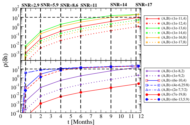
FIG. 2. \rho(\delta h) as a function of observation time. Observe that \rho(\delta h) > 5 within 1 year for a large set of (A, B) .
