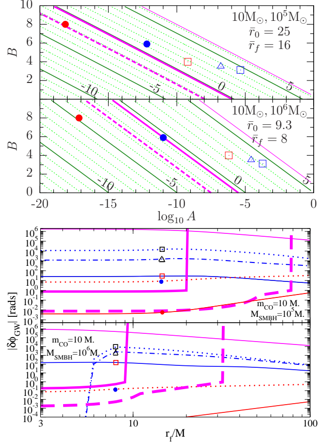
FIG. 1. Top: contours of \log_{10} |\delta\phi_{\text{GW}}| for different interaction models of two EMRI systems observed for one year. The symbols represent the models in Table I. Bottom: |\delta\phi_{\text{GW}}| versus \bar{r}_f for the 5 models in Table I [Type-I, \alpha ( \beta ) in solid (dotted) red, Type-II \alpha in solid blue, Type-II \beta of [19] and [20] in dotted and dot-dashed blue respectively]. The symbols represent the EMRIs considered in [10]. Many of the models – especially those resembling \beta -disks and Type II migration – shown in Table I lie well above the LISA sensitivity level [thick solid (optimistic) and dashed (pessimistic) magenta lines].
