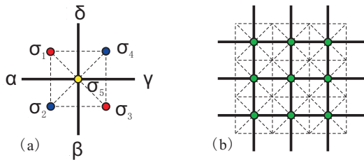
FIG. 2: (a) Schematic representation of the tensor T , obtained by integrating over the C-sublattice sites and performing the dual transformation. (b) The Union-Jack lattice (dashed lines) is transformed to the dual square lattice (solid lines) on which the tensor T is defined.
