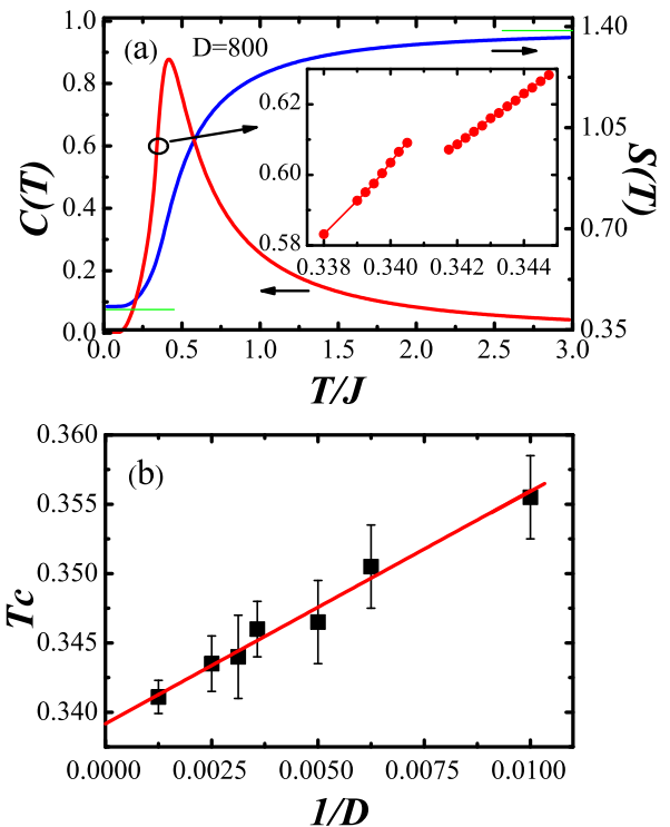
FIG. 3: (color online) (a) Entropy and specific heat for the q = 4 Potts model on the Union-Jack lattice, computed with D = 800 . Thin, green lines denote the zero- and infinite-temperature limits of the entropy. Inset: specific-heat discontinuity near T_c . (b) Linear fit of T_c with 1/D , which extrapolates to T_c(\infty) = 0.339(1) . The error bar denotes the upper and lower temperatures at the discontinuity.
