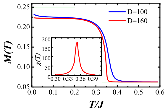
FIG. 5: (color online) Magnetization M(T) of sublattice A for the q = 4 Potts model on the Union-Jack lattice, calculated for an applied field of 0.000025. Thin green lines indicate the low- and high- T bounds. Inset: magnetic susceptibility \chi(T) .
