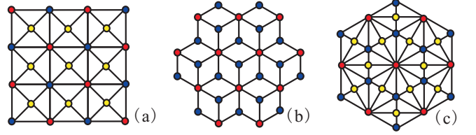
FIG. 1: (Color online) (a) Union-Jack lattice. Sites in sublattices A (red circles) and B (blue) have coordination numbers z_A = z_B = 8 , while those in sublattice C (yellow) have z_C = 4 . (b) Diced lattice. A sites (red) have z_A = 6 , while B sites (blue) have z_B = 3 . (c) Centered diced lattice: z_A = 12 (red), z_B = 6 (blue), and z_C = 4 (yellow).
