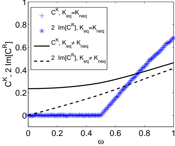
FIG. 1. C^K(q = 0.5, \omega) and 2\text{Im}[C^R(q = 0.5, \omega)] in equilibrium K_{eq} = K_{neq} = 2.0 and after a quench K_{eq} = 2, K_{neq} = 3
