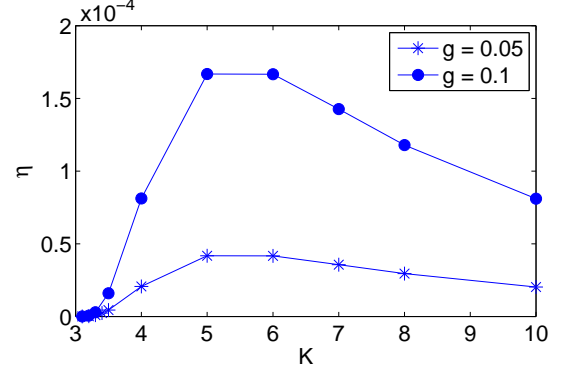
FIG. 2. Strength of the dissipation \eta for K_0=3 , \gamma=2 and g=0.05 and g=0.1 .
