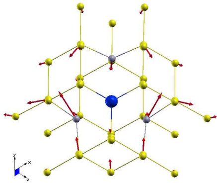
FIG. 3: Displacement vector associated with one of the local minima. Only atoms near the NV center are shown for clarity. Grey is for the carbons near the vacancy, yellow is for the other carbons, and blue is for nitrogen.
