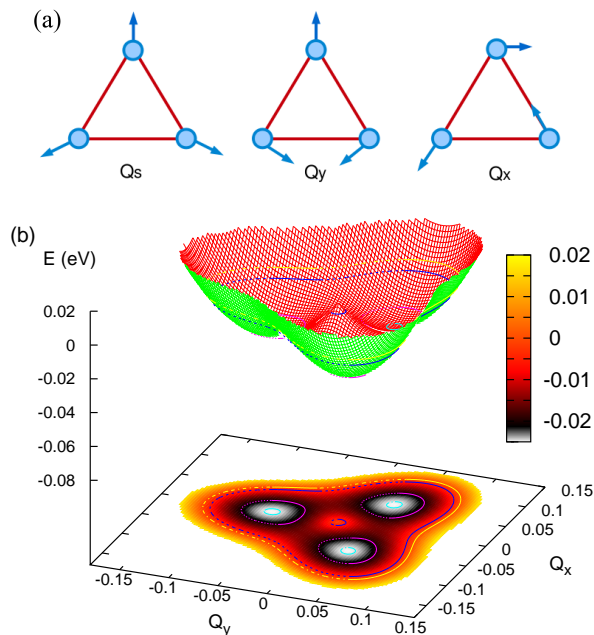
FIG. 2: (a) Three normal modes of a structure with the C_{3v} symmetry: totally symmetric displacement mode, Q_s ( a_1 type) and degenerate Q_x and Q_y modes ( e type). (b) The adiabatic potential energy surface for the NV^- center in diamond.
