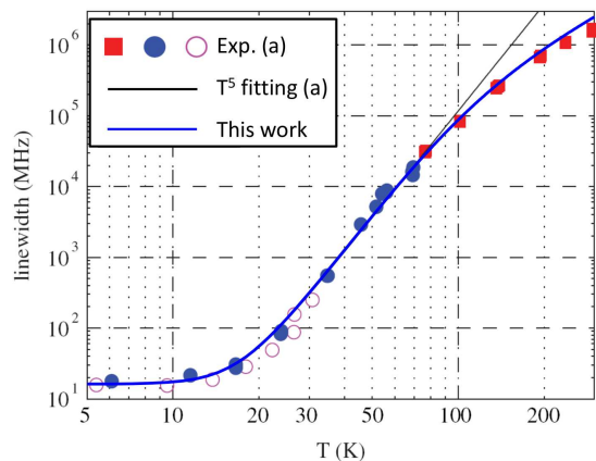
FIG. 4: Comparison between the calculated and the measured linewidth of the ZPL of the NV - center in diamond. (a) Experimental results and the T^5 fitting are taken from Ref. [11].
