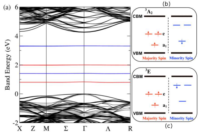
FIG. 1: (a) Band structure of the ground state of the NV - center in diamond. (b) Schematic one electron energy levels of the ground state ( 3 A 2 ). (c) Schematic one electron energy levels of the excited state ( 3 E).
