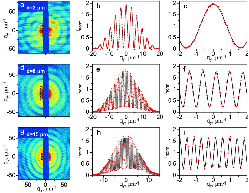
FIG. 2: (Color online) Measured diffraction patterns. Left column: Interference fringes from pinholes separated by 2 \mu\text{m} (a), 8 \mu\text{m} (d) and 15 \mu\text{m} (g) each exposed to a single shot of the LCLS beam as a function of the transverse momentum transfer q_x , q_y . The area used for the analysis of the transverse coherence is shown by the dashed black rectangle. Middle column: Line scans of the interference fringes on the right edge of the marked region, experimental data (red dots) and results of the theoretical fit (black lines). Right column: enlarged regions of the line scans shown in the middle column.
