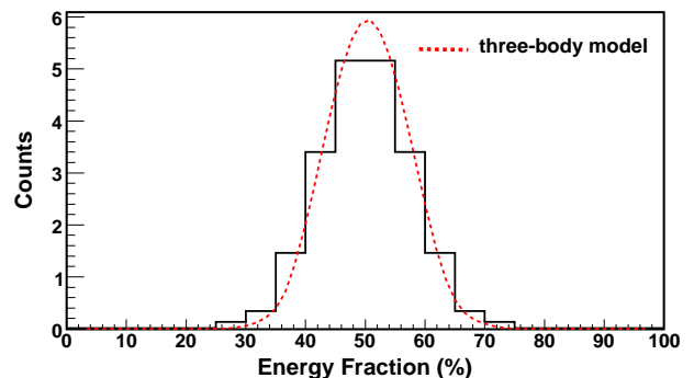
FIG. 4: Energy sharing between the two protons emitted in the decay of ^{54}\text{Zn} . The dashed line is the energy distribution of the three-body model [10] folded with the response of the detector, which fits well the experimental distribution.
