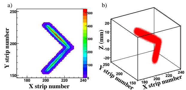
FIG. 3: a) Two-dimensional view of a ^{54}\text{Zn} decay event as reconstructed from the XY strip detector. The color corresponds to the energy loss detected by the strips. b) Same decay event reconstructed in the three-dimensional space.
