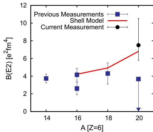
FIG. 3. (Color online) B(\text{E}2; 2_1^+ \rightarrow 0_{g.s.}^+) trend in even mass carbon isotopes for A = 16 –20 including only statistical errors. Previous data include ^{14}\text{C} [29], ^{16}\text{C} [8, 9], ^{18}\text{C} [9], ^{20}\text{C} [10]. We note that B(\text{E}2) values for ^{16}\text{C} [23] and ^{18}\text{C} [30] obtained at the NSCL using the same RDM technique as the current ^{20}\text{C} measurement agree well with the ^{16}\text{C} and ^{18}\text{C} B(\text{E}2) values plotted here. The red solid line is a shell model calculation discussed in the text.
