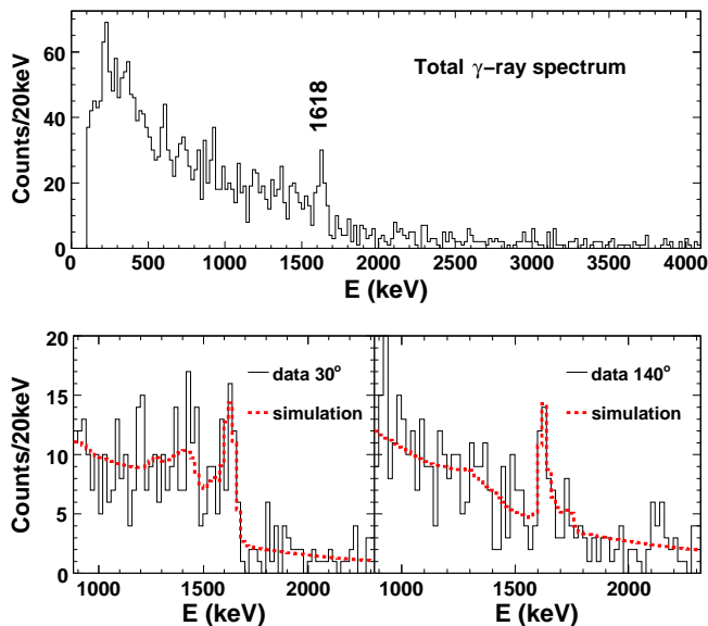
FIG. 1. (Color online) Top panel: Spectrum of \gamma rays, after Doppler correcting with v/c = 0.418 , obtained from a sum of all SeGA detectors and in coincidence with ^{20}\text{C} fragments. Lower panels: Spectra of \gamma rays for Ring 1 ( 30^\circ ) and Ring 2 ( 140^\circ ) after Doppler correcting with v/c = 0.418 . Experimental data are shown as a black solid line. Simulated data for \tau = 10 ps are shown as a red dotted line.
