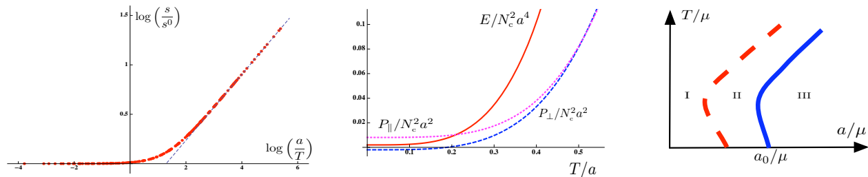
FIG. 1: (Left) Entropy density as a function of a/T . (Center) Energy and pressures as functions of T/a for fixed a \simeq 2.86 and \log \mu = 1/2 . (Right) Qualitative phase diagram.
