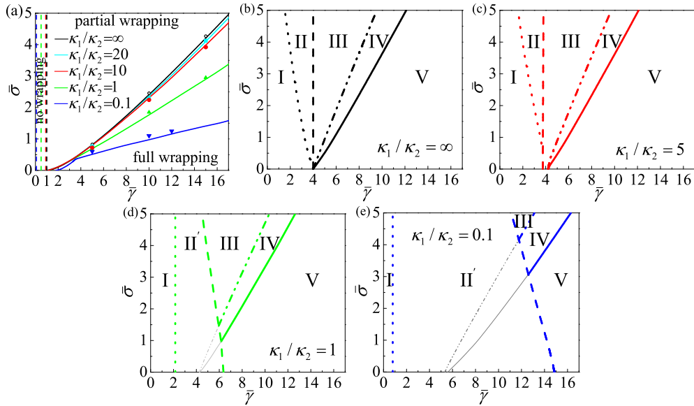
FIG. 3. (color online). Wrapping phase diagrams with respect to normalized adhesion energy \bar{\gamma} and surface tension \bar{\sigma} at different values of the rigidity ratio \kappa_1/\kappa_2 . (a) 2D case, dashed lines: boundaries between no wrapping and partial wrapping states, solid lines: boundaries between partial and full wrapping states. (b-e) 3D cases for \kappa_1/\kappa_2 = \infty, 5, 1, 0.1 , dotted lines: boundaries between phases I and II(II'), dashed lines: boundaries between phases II(II') and III(III-V for \kappa_1/\kappa_2 = 1, 0.1 ), dash-dotted lines: boundaries between phases III and IV, solid lines: boundaries between phases IV and V. Symbols in (a) denoting transition boundaries between the partial and full wrapping states are from molecular simulations [14].
