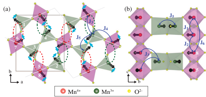
FIG. 3: Crystal and magnetic structures in the LTI phase of \text{YMn}_2\text{O}_5 projected onto the (a) ab - and (b) bc -plane. Thin white lines indicate the antiferromagnetic chains along the a axis. Also shown are the exchange coupling constants J_1 - J_6 used to calculate the spin-wave spectrum. Black arrows indicate the spin directions for the numerically obtained ground state of the spin Hamiltonian Eq.(1). The light blue arrows in (a) represent the directions of the oscillating Mn spins in the optical phason mode. Green (red) ellipses show that the angle between neighboring spins is increased (decreased) by this mode.
