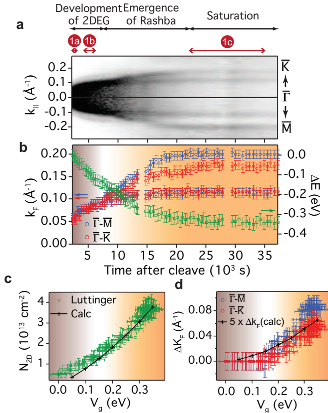
FIG. 4: (a) Evolution of the Fermi wave vector along \bar{\Gamma}-\bar{M} and \bar{\Gamma}-\bar{K} with time after cleaving the sample. (b) Extracted k_F positions and band-bending which induces the 2DEG. (c) Sheet density and (d) k_{||} -splitting at the Fermi level of the measured (points) and calculated (lines) Rashba-split 2DEG as a function of the effective gate potential, V_g .
