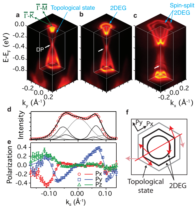
FIG. 1: (a–c) Electronic structure of Bi 2 Se 3 , measured using time-of-flight ARPES at increasing times (marked in Fig. 4(a)) after cleaving the sample ( h\nu = 19.2 eV, T = 10 K). (d) Spin-ARPES total intensity MDC at the Fermi level ( h\nu = 19.5 eV, T = 60 K) along the \bar{\Gamma} - \bar{M} direction, and (e) the measured (points) and fitted (lines) radial ( P_x ), tangential ( P_y ), and out-of-plane ( P_z ) components of the spin polarization along this cut. (f) Schematic representation of the in-plane component of the Fermi surface spin texture.
