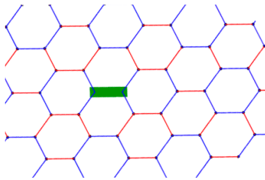
FIG. 5: Dimer-dimer correlation function, defined as in [4] for a SPS state. Green is the reference slice. Red indicates a positive correlation with the reference slice and blue a negative correlation. The SPS has the same positive and negative correlations as the dimer-dimer correlations found in [4].
