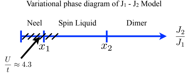
FIG. 1: Phase diagram of the quantum J_1 - J_2 model, obtained using the variational Monte Carlo method. As J_2/J_1 increases, the system undergoes a phase transition between an AFM state, and a gapped SL. We estimate the critical value of J_2/J_1 = x_1 \approx 0.08 . The arrow indicates the location for this transition in the Hubbard model [4]. The SL state is best described variationally by SPS. At higher J_2/J_1 = x_2 the SL gives way to a dimerized phase. Our variational study gives an estimate x_2 \approx 0.3 . Hashed area indicates values of J_2/J_1 that correspond to values of U/t in the Hubbard model that are in the Neel or SL state [4].
