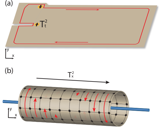
FIG. 1. (a) Chern insulator deformed by a dislocation - antidislocation pair, separated in the y -direction. For each dislocation, the momentum-density is in the direction of the Burgers vector. (b) Chern insulator on a cylinder with a (non-uniform) dislocation threading the cylinder. Local displacements are shown by red arrows. This gives rise to a momentum-current response along the cylinder which carries a momentum component parallel to the Burgers vector of the threaded dislocation, i.e., parallel to the red arrows.
