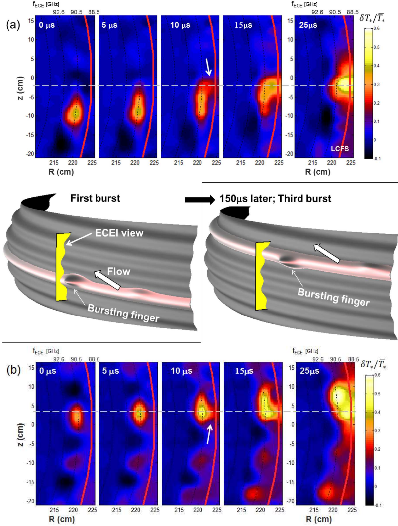
FIG. 4. (color online) Examples of multiple bursts of the same filament in a large ELM crash event. (a) First burst in the series of four bursts. Bottom left sketch depicts the phenomenological model for multiple localized bursts, showing the flux surface with the filamentary perturbations and the burst zone entering the ECEI view. Note that the filaments move in both toroidal and poloidal directions with respect to the laboratory frame (ECEI view) as indicated by the white box arrow. (b) Third burst of the same filament, 150 \mu\text{s} later. Top right sketch is the corresponding model. In each example, the bursting filament develops a narrow finger-like structure bulging outward.
