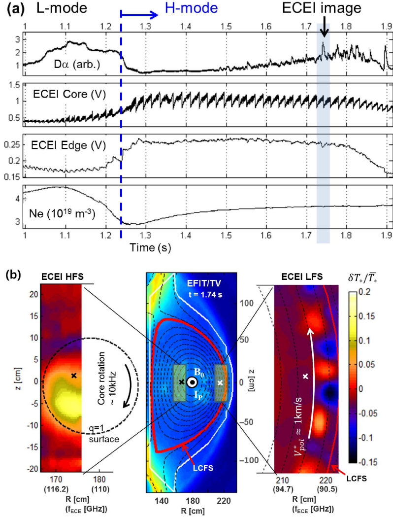
FIG. 1. (color online) (a) Time evolution of D_\alpha emission (from the lower central divertor), core ECEI signal, edge ECEI signal, and line-averaged n_e for ELMy H-mode plasma (shot no. 4362). (b) ECEI snapshot showing the core m/n = 1/1 internal kink (left) and the edge filaments (right). The poloidal rotation of the edge filaments is in opposite direction to the core rotation. The crosses are the approximate positions of the two ECEI channels. The radial coordinates are shown together with the corresponding cold resonant ECE frequencies ( f_{ECE} ). The middle figure depicts EFIT reconstructed flux surfaces overlaid on top of a fast visible camera image with the inset rectangles corresponding to the HFS (left) and LFS (right) ECEI views. The directions of B_0 and I_p are both out of the plane.
