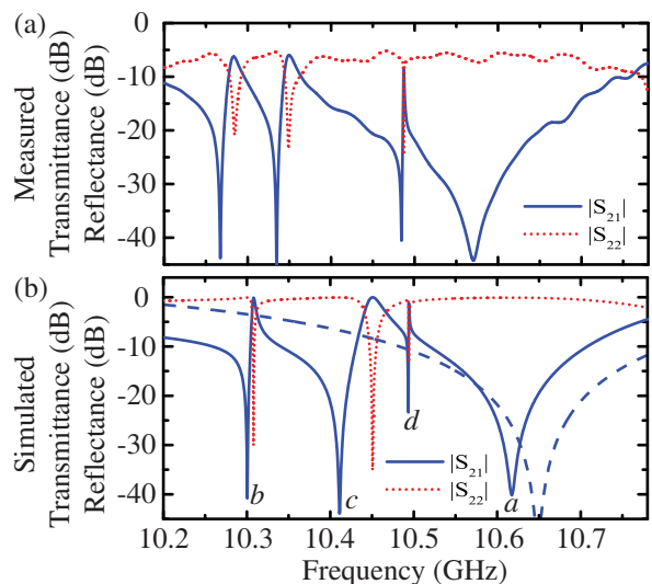
FIG. 1: (Color online) Transmittance and reflectance spectra. The transmittance shows a broad stopband originating from the coupling of the electromagnetic waves to the electric dipole mode of the wire, and three narrower resonance-like features that are associated with dark modes of the SRRs. (a) Experimental data at T = 2.6 K. The FWHM bandwidth of the resonant features is 9, 10, and 1 MHz for the transmittance peaks and 2, 1, and 0.1 MHz for the reflectance features. (b) Simulation data when the metamolecule is horizontally displaced by 0.1 mm from the center of the waveguide. The dashed blue line is a simulation of the wire only. The labels a-d correspond to the current distributions in Fig. 2.
