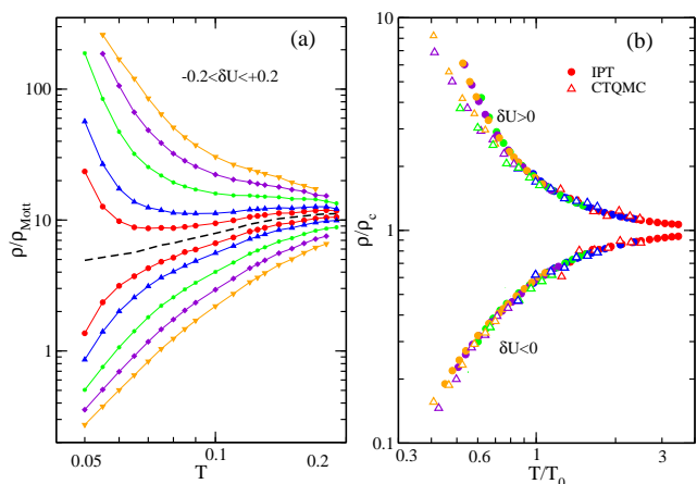
Figure 1: (Color online) (a) DMFT resistivity curves as function of temperature along different trajectories -0.2 \leq \delta U \leq +0.2 with respect to the instability line \delta U = 0 (black dashed line, see the text). Data are obtained using IPT impurity solver. (b) Resistivity scaling; essentially identical scaling functions are found from CTQMC (open symbols) and from IPT (closed symbols)
