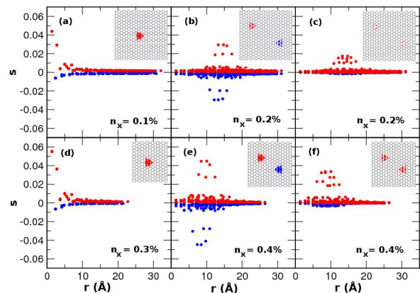
FIG. 2: (color online) Local (site) spin ( s ) versus r (the distance to the center of the supercell) for various vacancy concentrations: (a,d) n_x = 0.1\% and 0.3\% in the paramagnetic case, (b,e) n_x = 0.2\% ( d = 27.7\text{Å} ) and 0.4\% ( d = 18.1\text{Å} ) in an antiferromagnetic state, and (c,f) in a ferromagnetic excited state within the mean-field Hubbard approximation [ \uparrow (red) and \downarrow (blue) electrons]. In all cases, the center of mass of the vacancies is at r = 0 .
