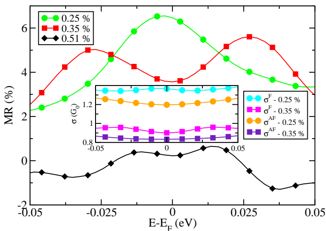
FIG. 4: (color online) Magnetoresistance of hydrogenated graphene samples with concentrations of n_x = 0.25, 0.35, 0.5\% as a function of charge energy. Inset : Conductivities for the ferromagnetic and antiferromagnetic graphene samples at densities of n_x = 0.25, 0.35\% .
