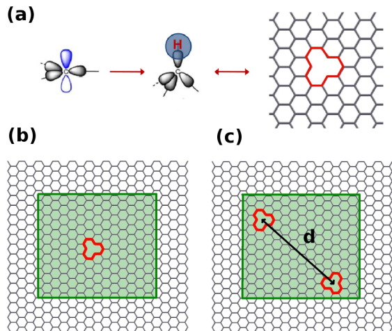
FIG. 1: (color online) (a) Schematic representation of the sp^2 hybridization breakdown upon hydrogen adsorption. In our tight-binding model, such a defect can be mimicked by a monovacancy. (b) Single-vacancy supercell used in the mean-field Hubbard model calculations with periodic boundary conditions. (c) Supercell with two vacancies. The distance between two hydrogen defects is labeled by d . The green colored region give the space location for the defects, to minimize the correlations between vacancies in neighboring cells.
