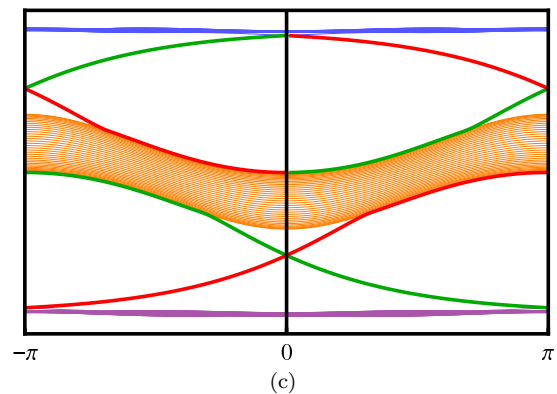
FIG. 1: (Color online) Chiral quasi-flat band in the three-band model on a square lattice. Figure (a) shows the lattice structure, where each lattice site contains three orbitals and the arrows represent the breaking of the time-reversal symmetry. By putting the system on a torus and a cylinder, the single-particle energy spectra are shown in Figs. (b) and (c). In Fig. (c), chiral edge states (thick lines) are observed.
