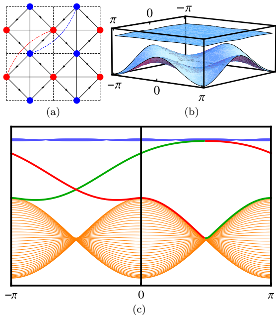
FIG. 2: (Color online) Chiral quasi-flat band on the checkerboard lattice. The lattice structure is shown in Fig.(a), with arrows and (solid and dashed) lines representing the NN and NNN hoppings respectively. The direction of the arrow shows the sign of the phase in the NN hopping terms. Two of the NNN hoppings are shown as the dashed curve. Other convention are the same as in Fig. 1.
