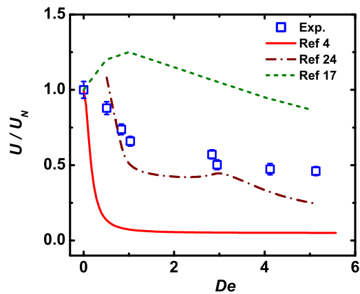
FIG. 3. Color Online. Swimming speed normalized by Newtonian speed ( U_N ) as a function of Deborah number ( De ). The data (squares) show that propulsion speed decreases as elasticity in the fluid increases. The solid and dashed lines are the theoretical predictions of [4] and [24], respectively, and the dotted line is the numerical simulation of [17].
