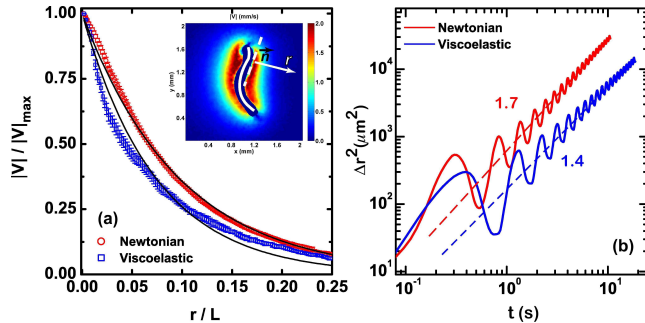
FIG. 4. Color Online. (a) Velocity decay normal to the C. elegans swimming direction (inset) for Newtonian and viscoelastic cases ( De = 3.0 ) at Re < 10^{-3} . The fluid viscosity is \mu = 200 mPa·s. Lines corresponds to exponential fits (see text). (b) Mean square displacements of the Newtonian and viscoelastic fluids after 20 beating cycles T .
