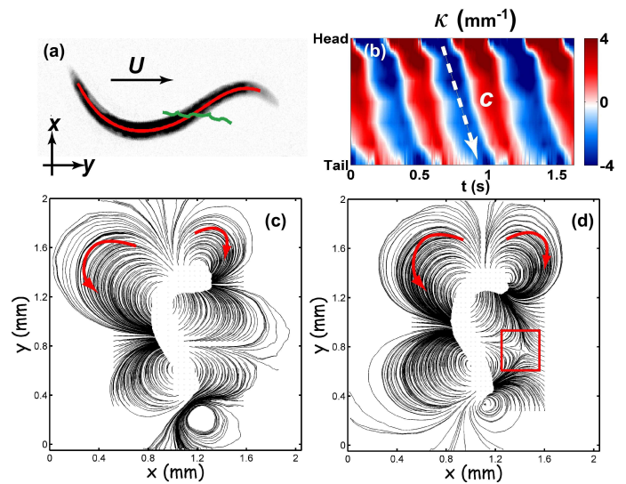
FIG. 1. Color Online. (a) Sample snapshot of the nematode C. elegans swimming in buffer solution ( \mu = 1.0 mPa·s). The red line represents nematode's “skeleton” while the green line represents its centroid path. (b) Corresponding contour plots of the nematode's bending curvature \kappa(s, t) over 3 swimming cycles. Red and blue colors correspond to positive and negative \kappa values, respectively. (c) Streamlines computed from instantaneous velocity fields of Newtonian ( Re < 10^{-3} ) and (d) polymeric ( Re < 10^{-3} ; De = 3.0 ) fluids. Arrows in (c,d) indicate flow direction and the box in (d) shows a hyperbolic point in the flow.
