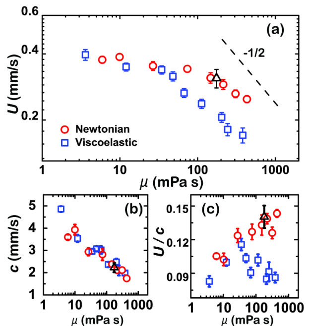
FIG. 2. Color Online. (a) Swimming speed, (b) bending wave speed, and (c) kinematic efficiency of C. elegans in Newtonian (red circle) and viscoelastic (blue square) fluids as a function of fluid viscosity. Triangle symbol represents the non-elastic Xanthan Gum solution. The data shows that fluid elasticity decreases the nematode's swimming speed and efficiency when compared to a Newtonian fluid of same viscosity. For \mu > 30 mPa-s, the nematode's swimming speed decreases indicating a limit in power for this type of organism.
