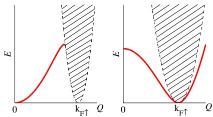
FIG. 2: (Color online) Schematics of two scenarios for a molecule unbinding into a polaron + particle. The solid (red) lines represent the molecule dispersion E(Q) and the shaded regions correspond to the polaron + particle (two-body) continuum. When both the molecule and polaron have their minimum energies at \mathbf{Q} = 0 (left), the transition is first-order. However, we have a continuous transition (where the bound state fully “mixes” with the continuum) when the molecule has ground-state momentum Q = k_{F\uparrow} (right).
