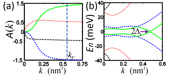
Figure 2. (Color online) (a) Plot of A(k) with respect to k . (b) Plot of the bulk quasiparticle energy E_n of Eq. (9). Solid, dashed, dotted, and dashed dotted lines correspond to the lowest to the highest bands in Fig. 1b. \mu = -32.5 eV. The other parameters are the same as that in Fig. 1.
