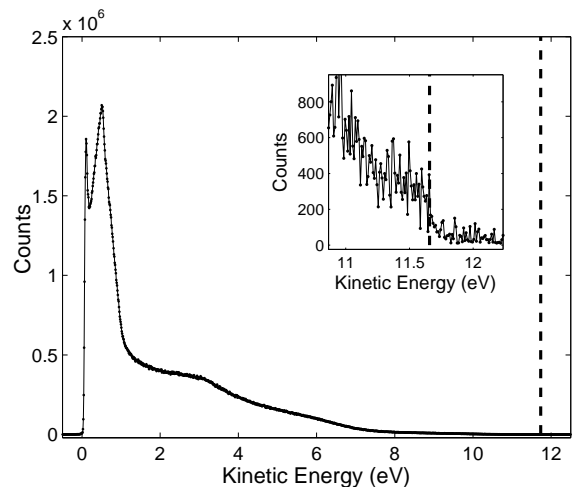
FIG. 1: Density of states for H:C(B)[100] at 16 eV photon energy. E_F is marked by the dashed line at 11.73 eV yielding a work function \phi = 4.27 eV. Inset: a zoom of the near- E_F spectrum. The kinetic energy has been corrected for the external bias and the offset imparted by the analyzer. Lines connecting points are a guide to the eye.
