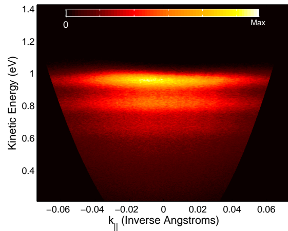
FIG. 2: ARPES spectrum acquired using the 6.01 eV laser. The color bar shows relative intensity. The overall “bowl” shape of the spectrum results from scaling between emission angle and k_{||} . (Color online)
