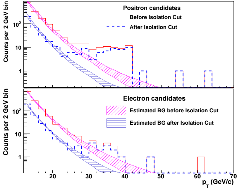
FIG. 1: (color online) The spectra of positron (upper panel) and electron (lower panel) candidates before (solid histogram) and after (dashed histogram) an isolation cut. The bands reflect the uncertainty of the background.
