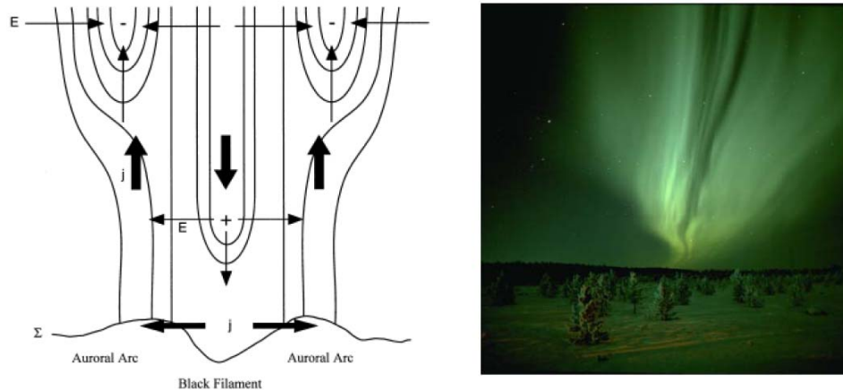
Figure 1. A schematic of the electric field and current system (left) representative of two parallel arcs (right) in upward current regions, separated by dark bands in regions of downward current. The arcs are produced by high-energy electrons colliding with the upper atmosphere, after being accelerated by an upward directed parallel electric field at altitudes around one Earth radius. Above the dark areas, a downward directed electric field accelerates electrons away from Earth, corresponding to a downward current. How the parallel electric fields and potential drops are distributed in altitude is studied here, for the first time using Cluster multi-probe data obtained at different heights of the AAR.
