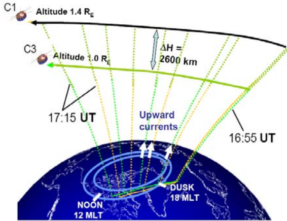
Figure 2. Schematic view of the Cluster C3 and C1 satellite trajectories between 16:55 and 17:15 UT on 5 June 2009, crossing the AAR of dusk-side aurora at altitudes of 1 and 1.4 R_E , respectively. The blue ovals indicate the poleward half of the auroral oval, which is characterized by upward and downward currents for the dusk-side and dawn-side magnetic local time sectors, respectively.
