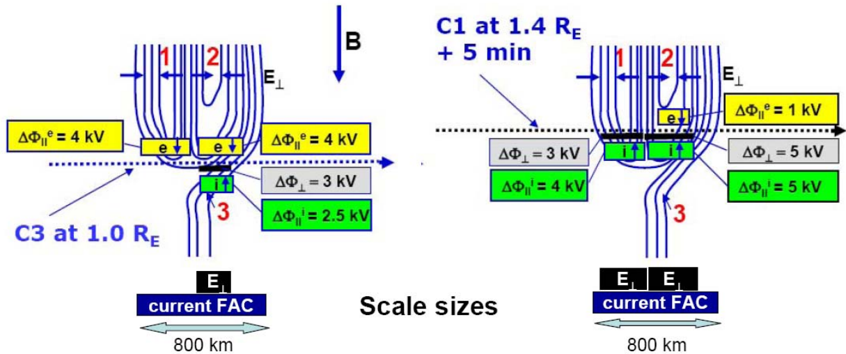
Figure 4. Altitude distribution of the acceleration potential, presented in terms of equipotential contours (spacing 1 kV), derived by combining Cluster 3 and 1 data. The pattern consists of two upper and broad U-shaped potential structures (1 and 2) and a narrower S-shaped potential structure (3) located below. The small boxes indicate the widths of the down-going electron (yellow) and up-going ion (green) distributions. The black bold lines in between, indicate where the electric potential deviated much from the ambient level. The larger attached boxes present acceleration potential estimates. For the region above the spacecraft, the acceleration potential, \Delta\Phi_{||}^e , is inferred from the down-going electron energy (yellow). For the region below the spacecraft, the acceleration potential is estimated from the potential drops, \Delta\Phi_{\perp} (grey), and from \Delta\Phi_{||}^i , given by the peak ion energy (green). The vertical potential drops remained stable at 4 kV at the position of structure 1, and between 6 and 7 kV at the position of structure 2. The total structure (or current) width also remained stable, 800 km for both spacecraft, scaled to their mean altitude. Note also that the scale size of the electric field relative to that of the current was much smaller on Cluster 3, but roughly equal for Cluster 1.
