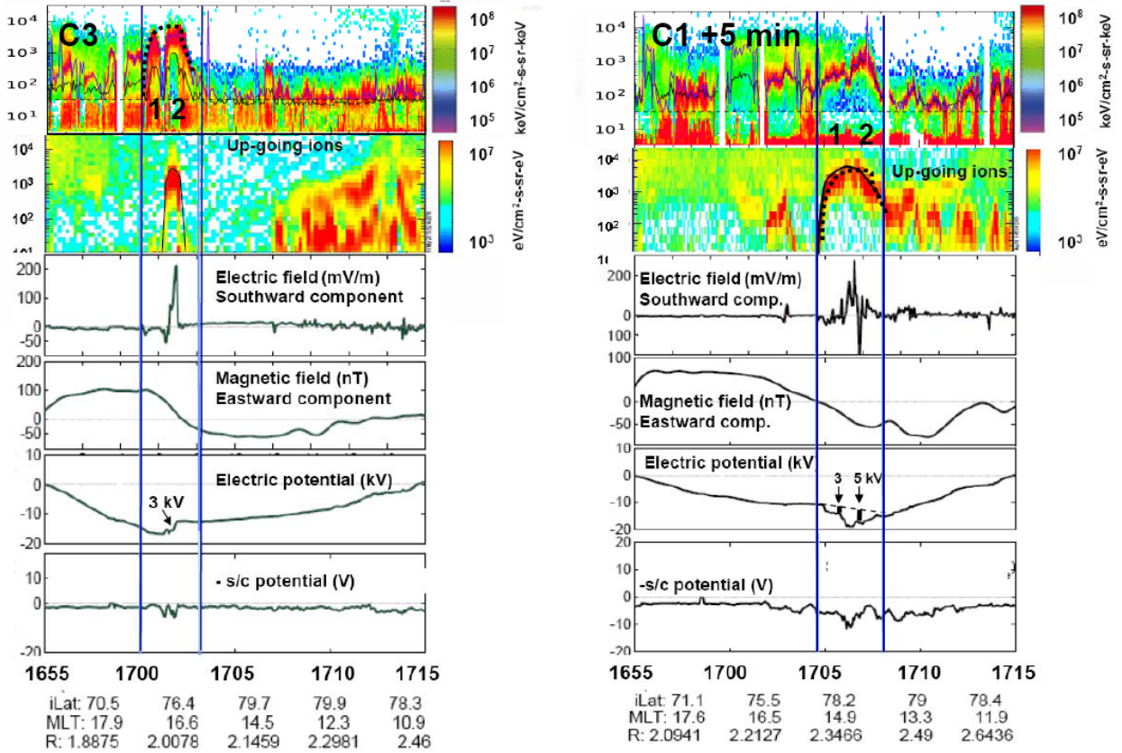
Figure 3. Cluster 3 data at 1 R_E (left) and Cluster 1 data at 1.4 R_E (right) between 16:55 and 17:15 UT. The panels show, from the top: (1) energy spectrograms of down-going electrons; (2) energy spectrograms of up-going ions, the peak energy given by the solid black curve; (3) the electric field component perpendicular to the geomagnetic field \mathbf{B} and normal to the oval, \sim the southward component; (4) the residual magnetic field component tangential to the oval, \sim the eastward component; (5) the potential, integrated from the electric field along the trajectory; (6) the negative of the spacecraft potential, indicating relative plasma density variations.
